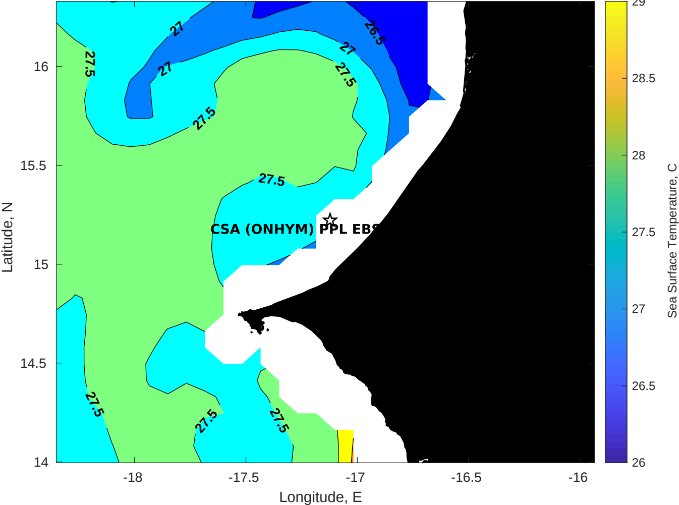
SST for CSA (ONHYM) PPL EBS - Senegal at 24-Jul-2025 00:00:00
