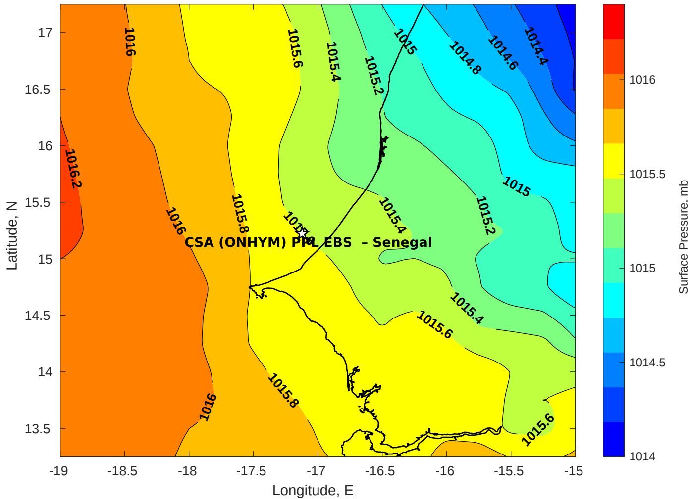
Surface Pressure (mb) for CSA (ONHYM) PPL EBS - Senegal at 27-Jul-2025 00:00:00
