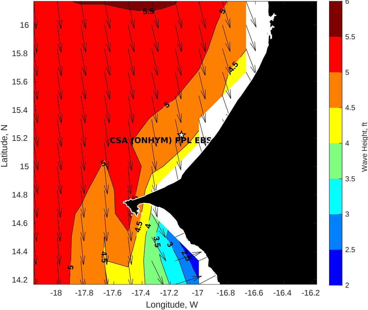
Wave Height (ft) for CSA (ONHYM) PPL EBS - Senegal at 25-Jul-2025 09:00:00
