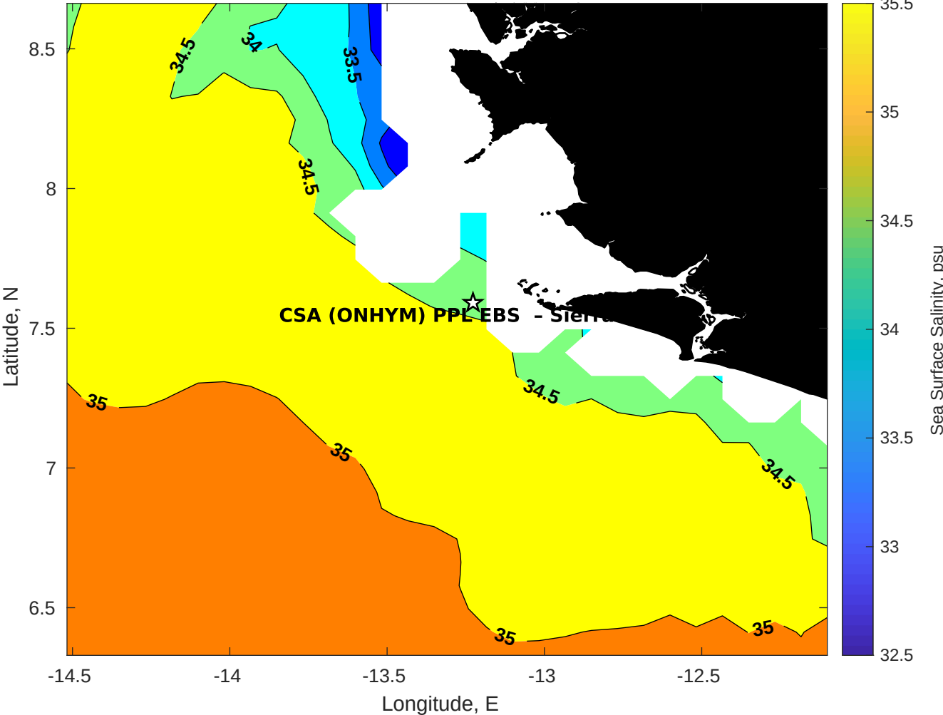
Surface Salinity for CSA (ONHYM) PPL EBS - Sierra Leone at 24-Jul-2025 00:00:00
