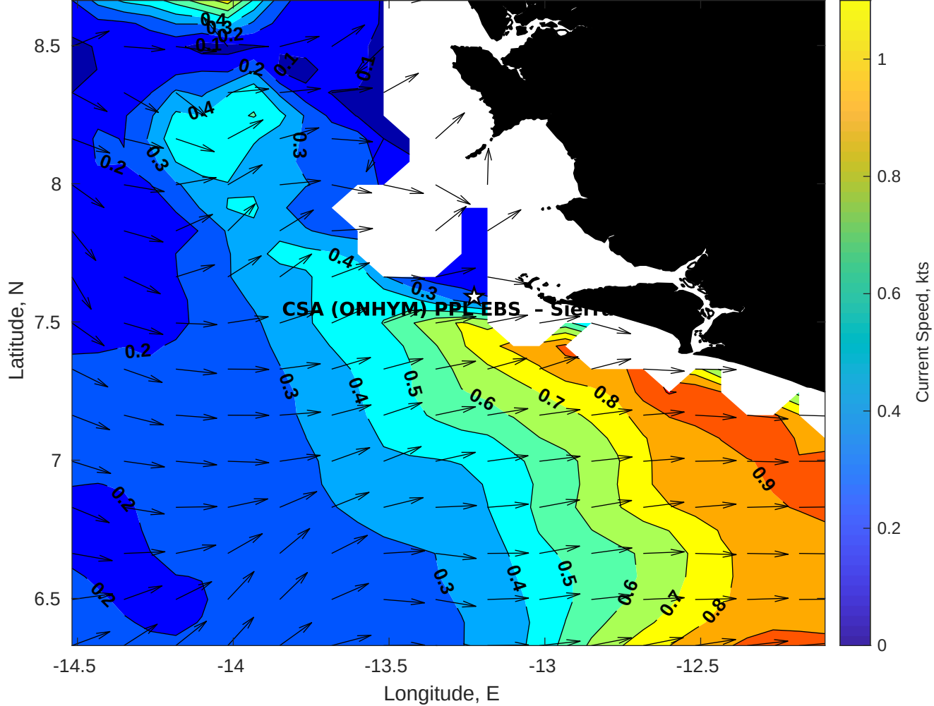
Surface Currents for CSA (ONHYM) PPL EBS - Sierra Leone at 24-Jul-2025 00:00:00
