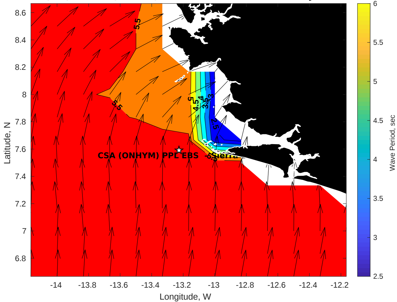
Wave Period (sec) for CSA (ONHYM) PPL EBS - Sierra Leone at 25-Jul-2025 09:00:00
