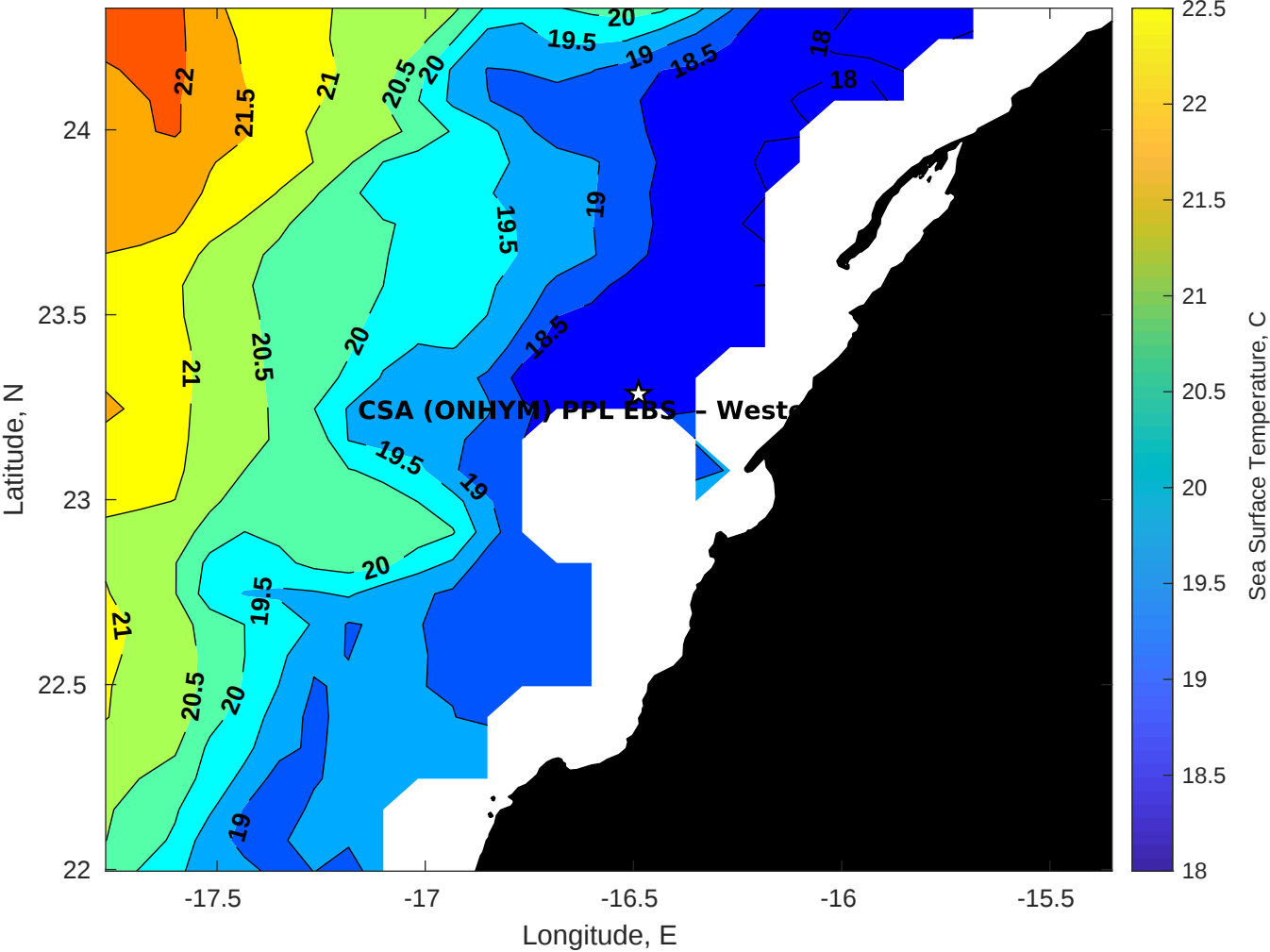
SST for CSA (ONHYM) PPL EBS - Western Sahara at 24-Jul-2025 00:00:00
