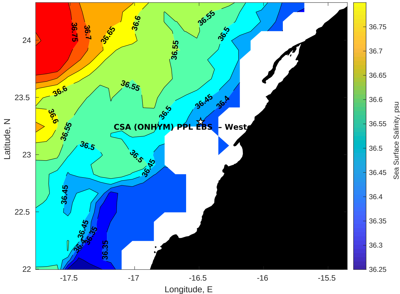
Surface Salinity for CSA (ONHYM) PPL EBS - Western Sahara at 24-Jul-2025 00:00:00
