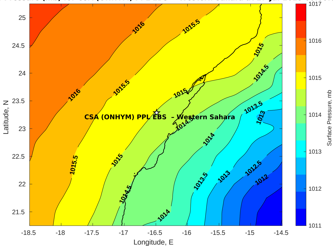
Surface Pressure (mb) for CSA (ONHYM) PPL EBS - Western Sahara at 27-Jul-2025 00:00:00
