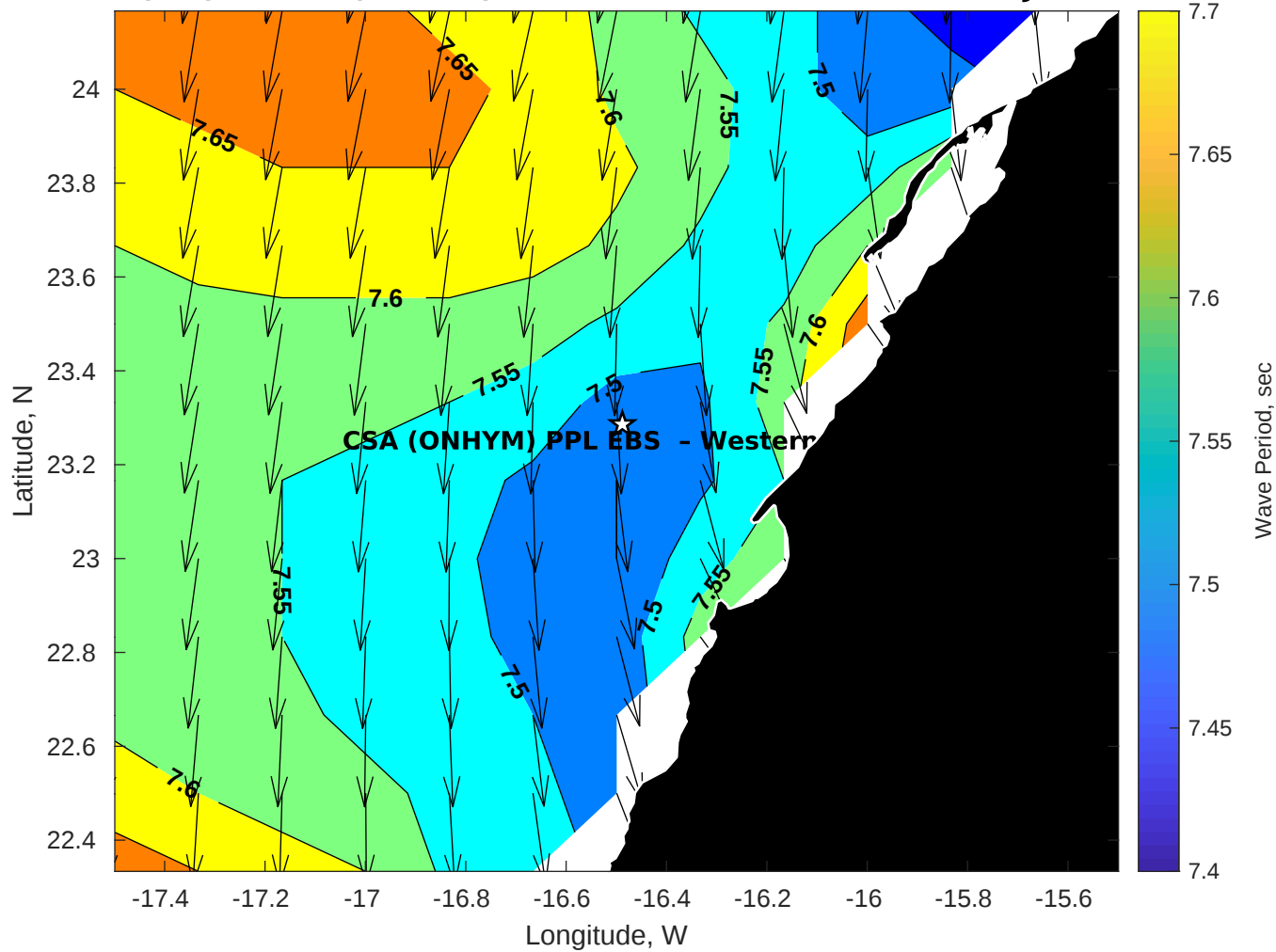
Wave Period (sec) for CSA (ONHYM) PPL EBS - Western Sahara at 25-Jul-2025 09:00:00
