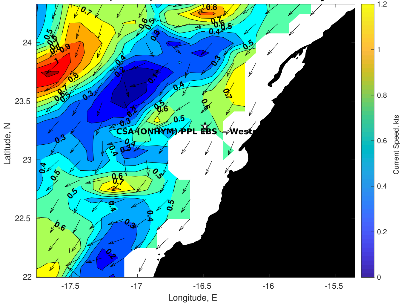
Surface Currents for CSA (ONHYM) PPL EBS - Western Sahara at 24-Jul-2025 00:00:00
