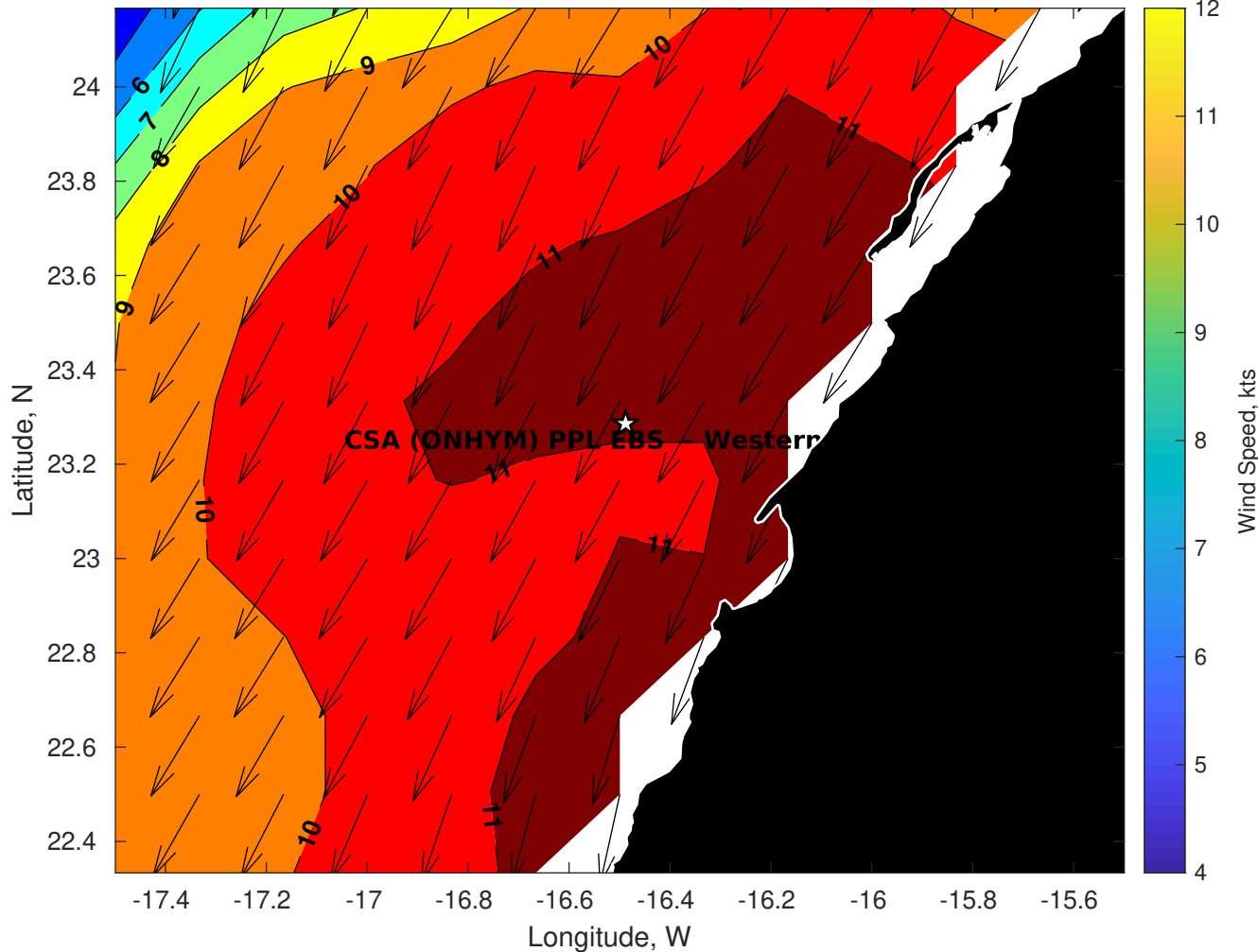
Winds (kts) for CSA (ONHYM) PPL EBS - Western Sahara at 25-Jul-2025 09:00:00
