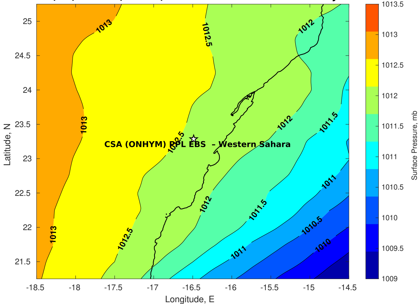
Surface Pressure (mb) for CSA (ONHYM) PPL EBS - Western Sahara at 25-Jul-2025 00:00:00
