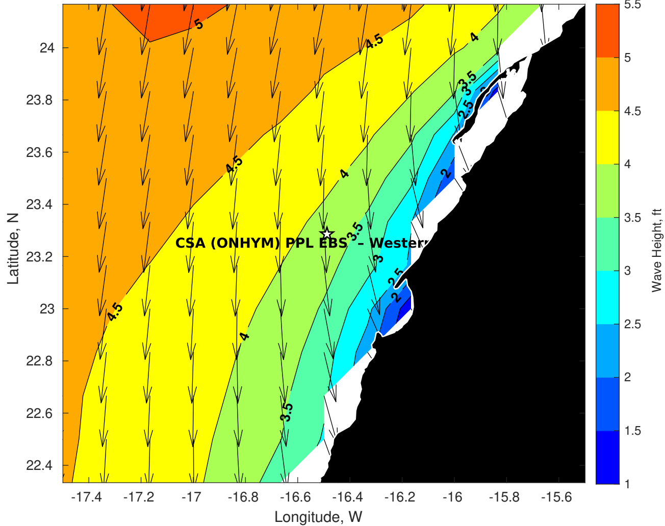
Wave Height (ft) for CSA (ONHYM) PPL EBS - Western Sahara at 25-Jul-2025 09:00:00
