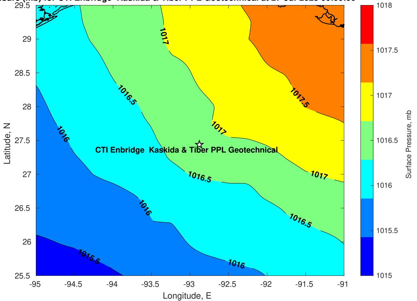
Surface Pressure (mb) for CTI Enbridge Kaskida & Tiber PPL Geotechnical at 27-Jul-2025 00:00:00
