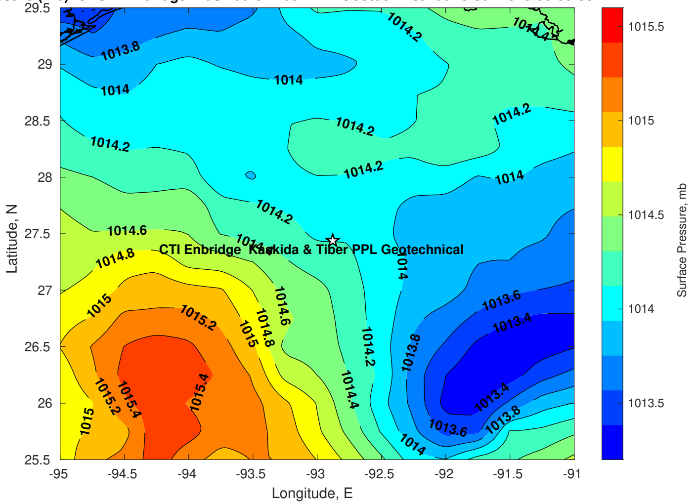
Surface Pressure (mb) for CTI Enbridge Kaskida & Tiber PPL Geotechnical at 25-Jul-2025 00:00:00
