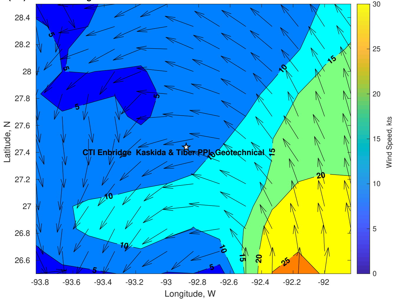
Winds (kts) for CTI Enbridge Kaskida & Tiber PPL Geotechnical at 25-Jul-2025 09:00:00
