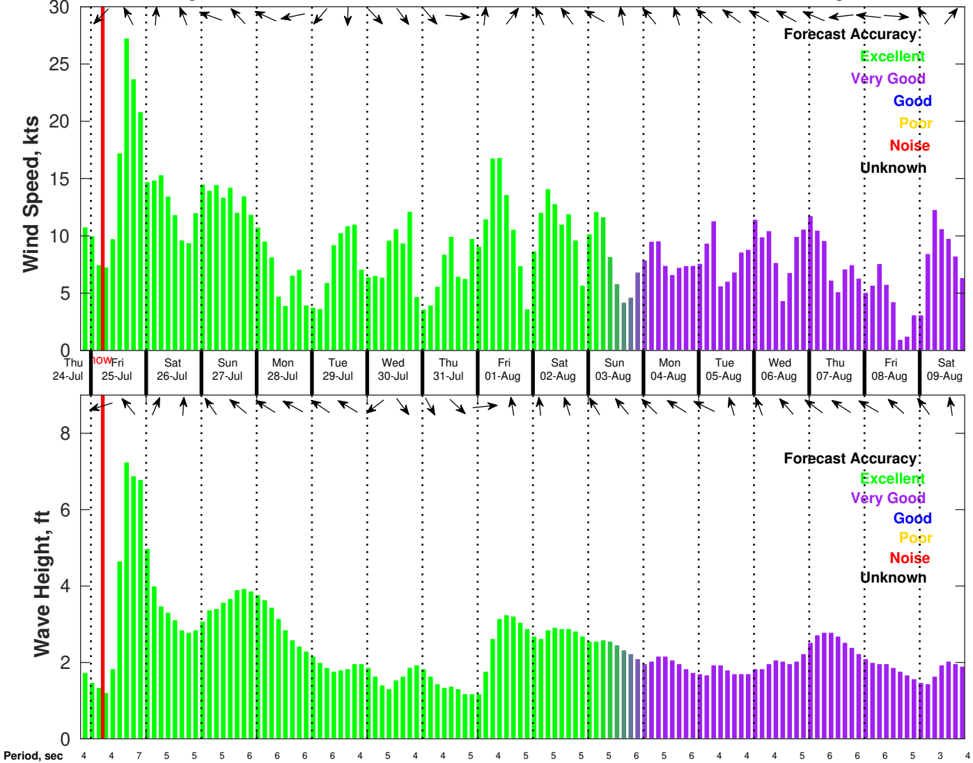
Wind & Wave Forecast for CTI Enbridge Kaskida & Tiber PPL Geotechnical from 24-Jul-2025 20:00:00 to 09-Aug-2025 20:00:00
