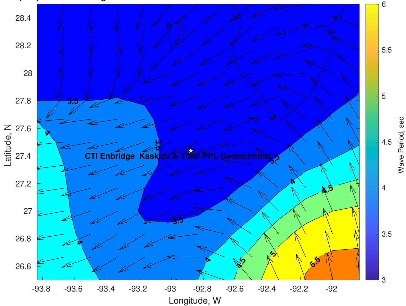
Wave Period (sec) for CTI Enbridge Kaskida & Tiber PPL Geotechnical at 25-Jul-2025 09:00:00
