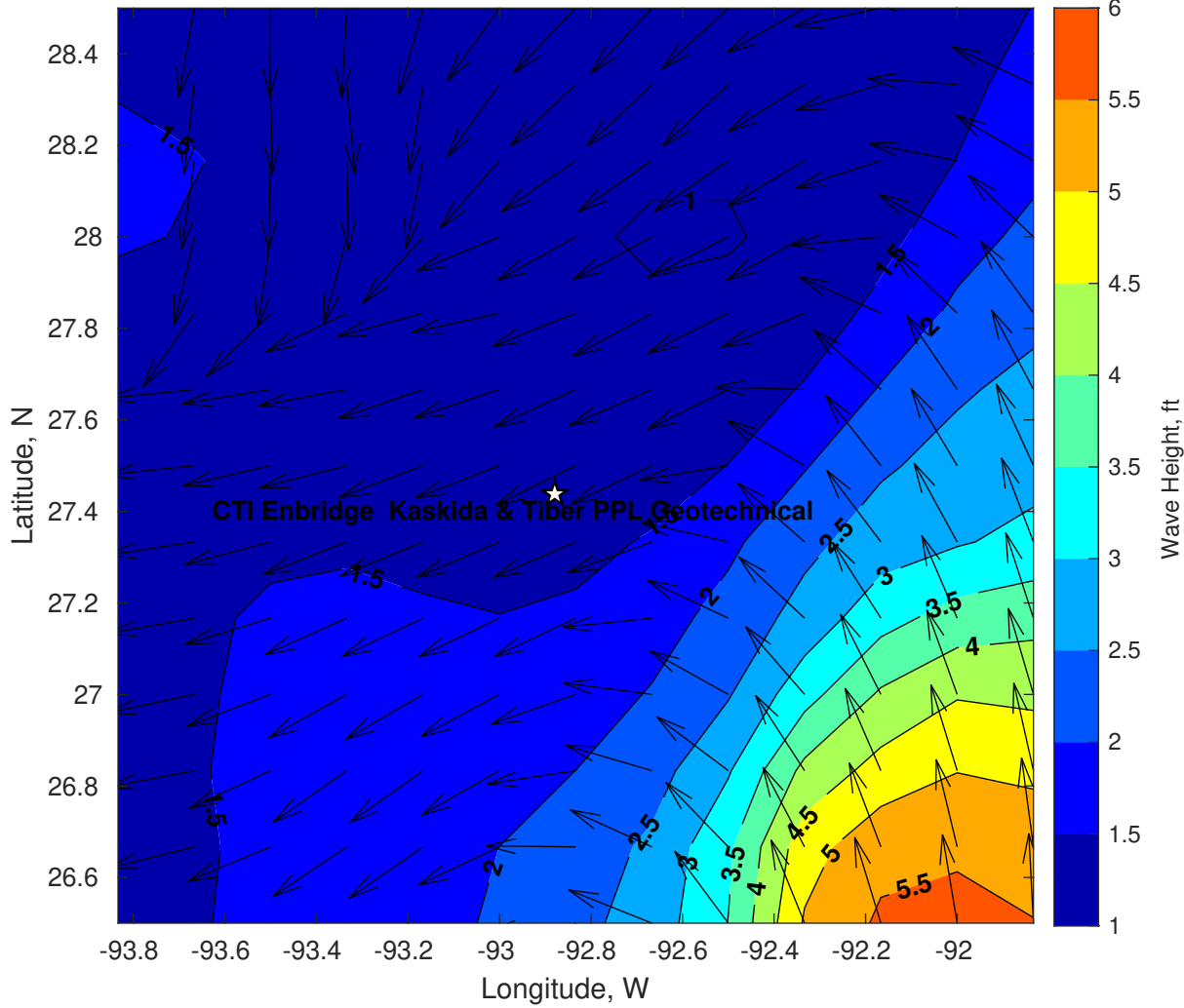
Wave Height (ft) for CTI Enbridge Kaskida & Tiber PPL Geotechnical at 25-Jul-2025 09:00:00
