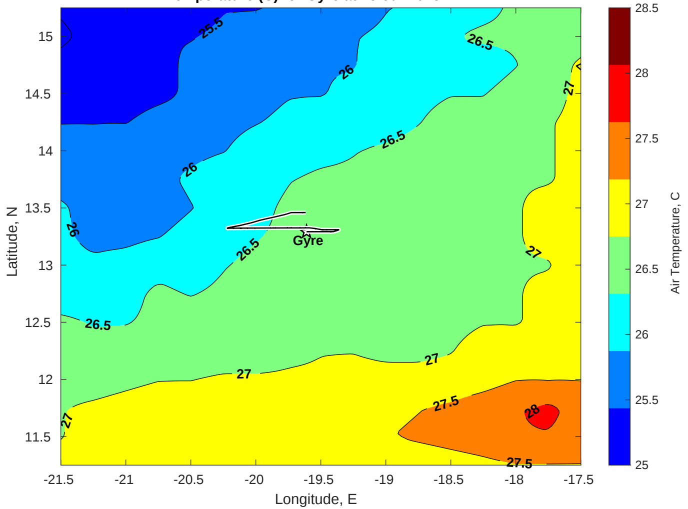
Air Temperature (C) for Gyre at 25-Jul-2025
