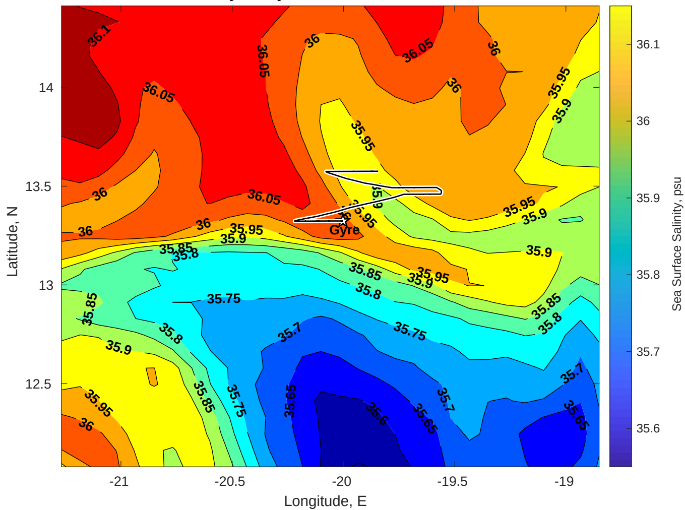
Surface Salinity for Gyre at 24-Jul-2025 00:00:00
