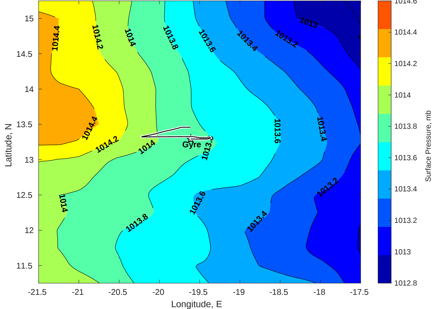
Surface Pressure (mb) for Gyre at 25-Jul-2025 00:00:00
