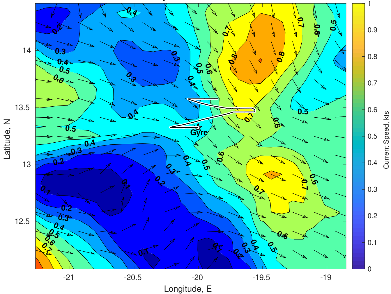
Surface Currents for Gyre at 24-Jul-2025 00:00:00
