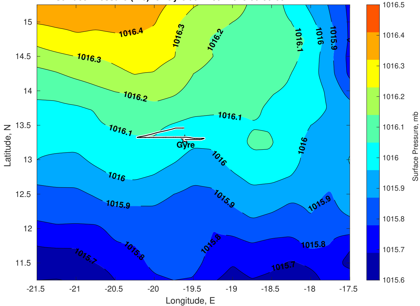
Surface Pressure (mb) for Gyre at 27-Jul-2025 00:00:00
