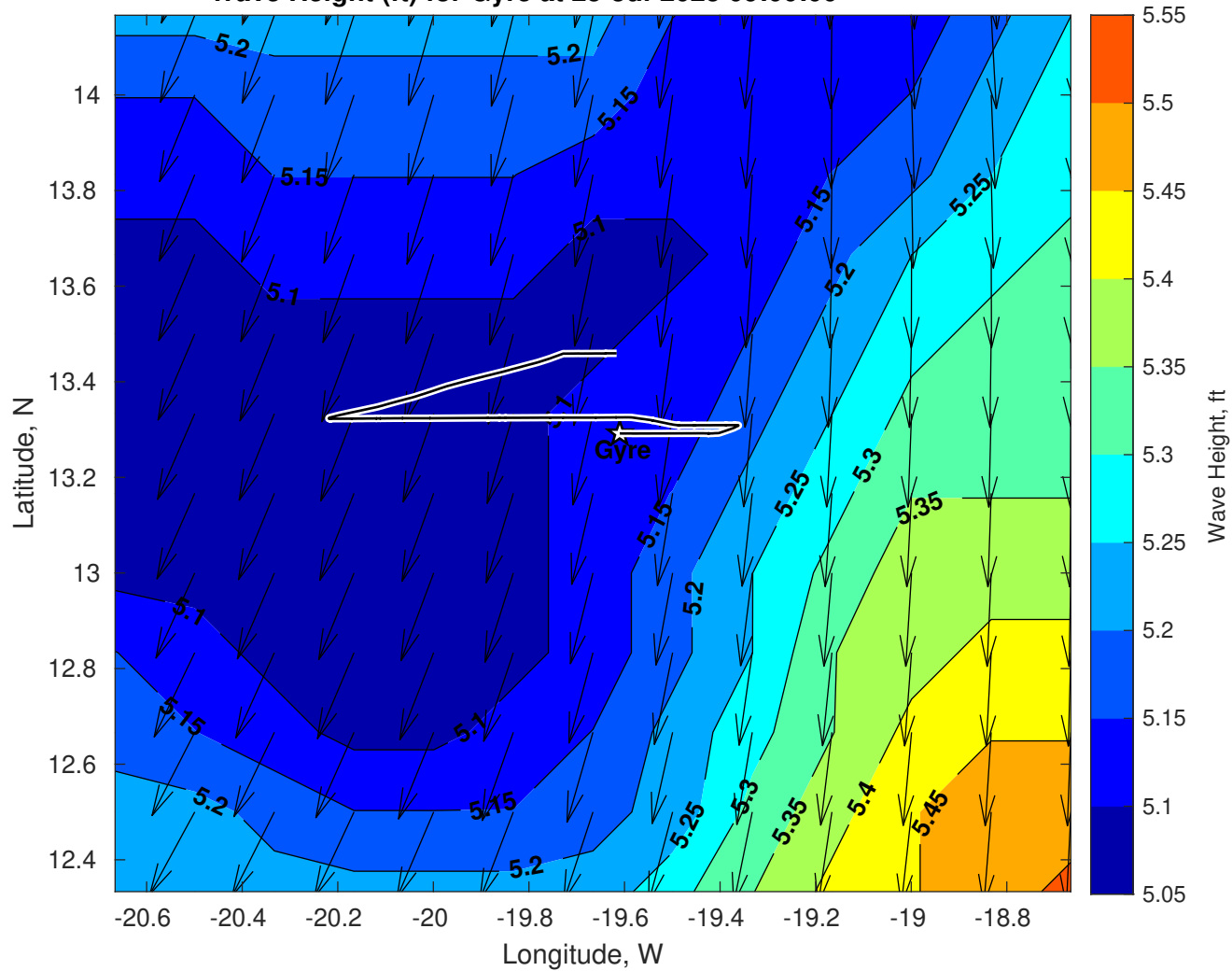
Wave Height (ft) for Gyre at 25-Jul-2025 09:00:00
