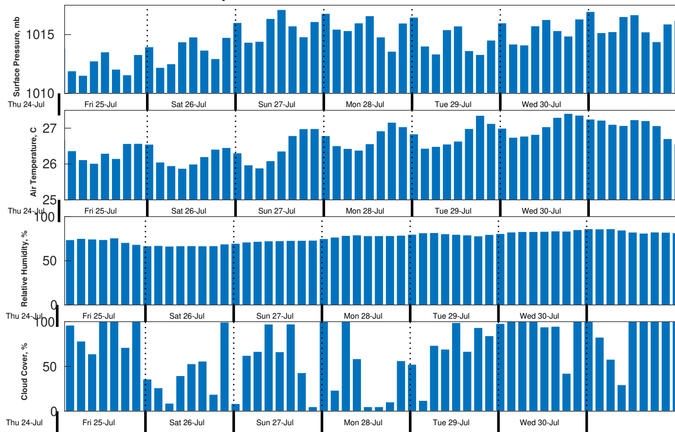
Met Forecast for Gyre from 24-Jul-2025 23:00:00 to 31-Jul-2025 23:00:00
