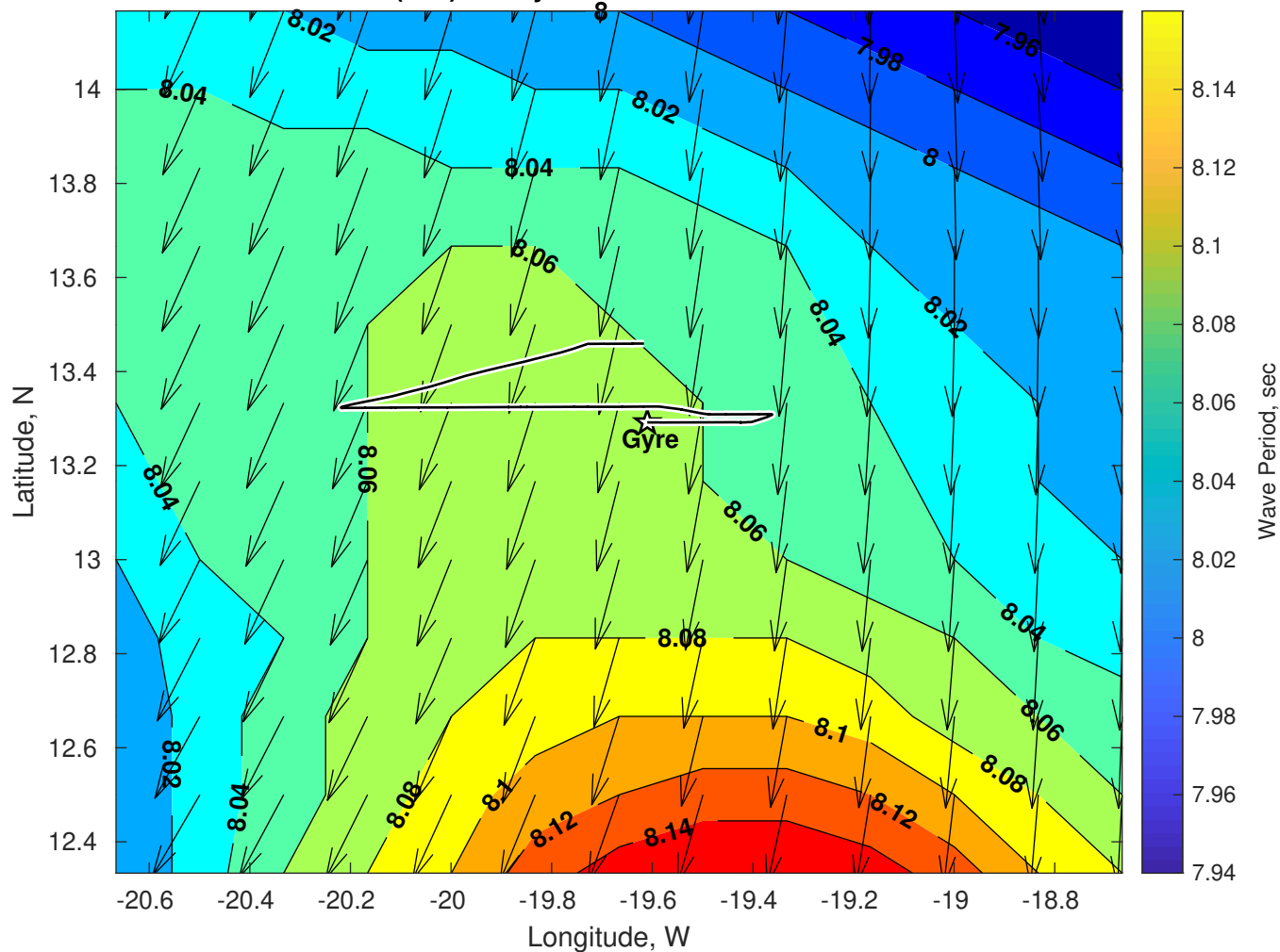
Wave Period (sec) for Gyre at 25-Jul-2025 09:00:00
