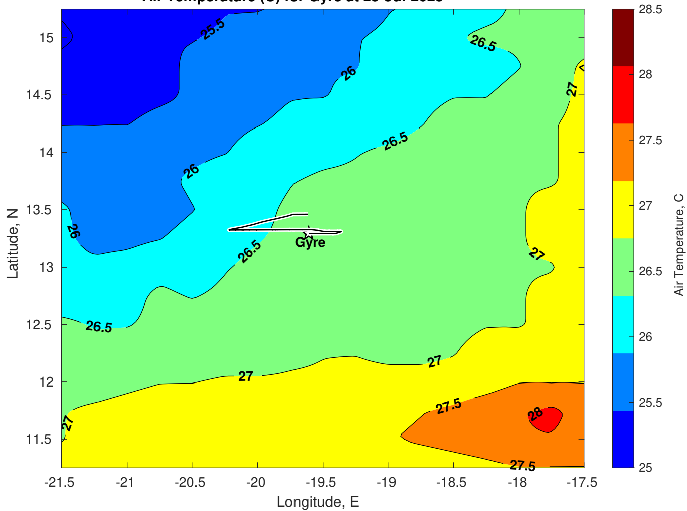
Air Temperature (C) for Gyre at 25-Jul-2025
