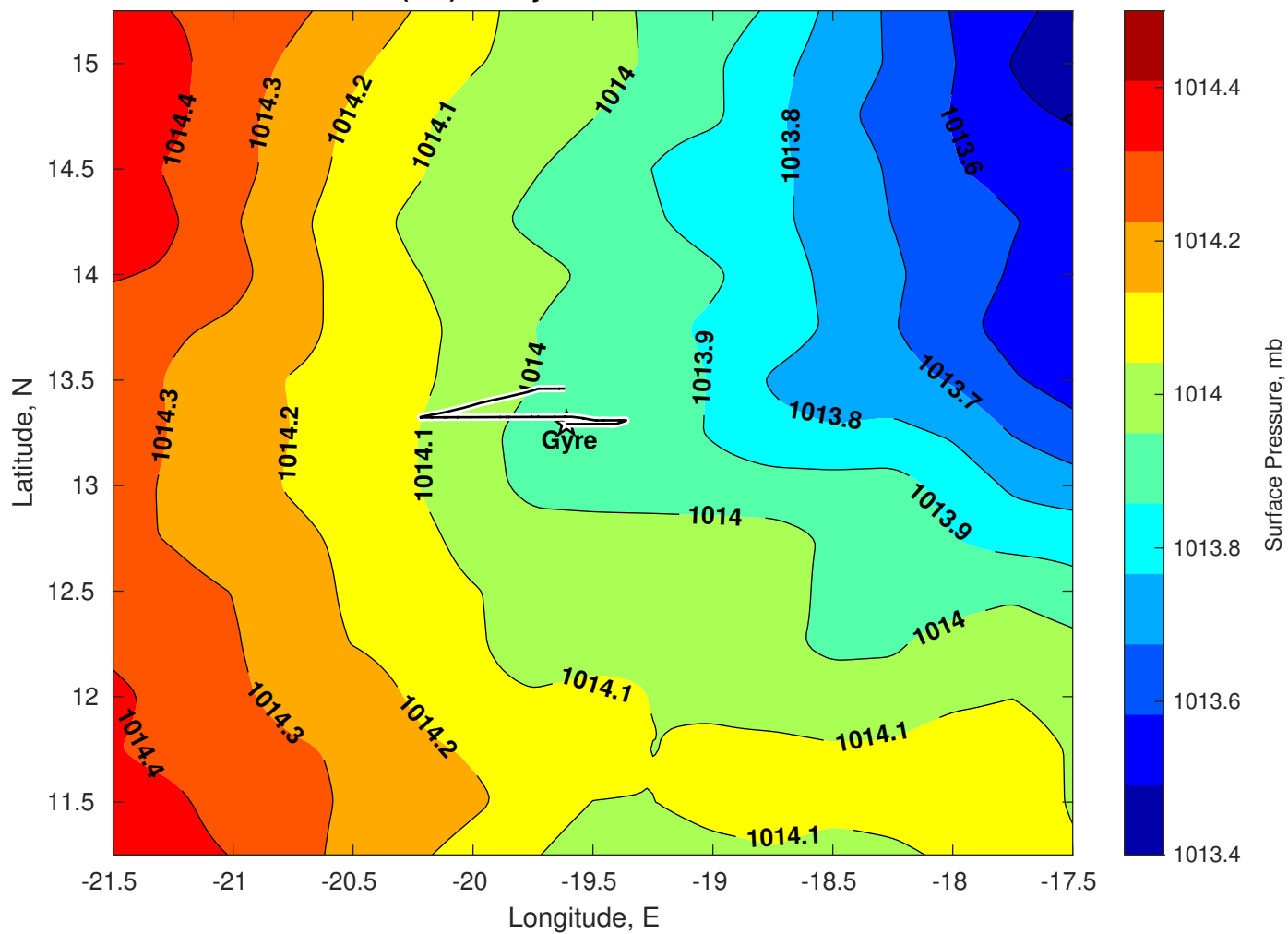
Surface Pressure (mb) for Gyre at 26-Jul-2025 00:00:00
