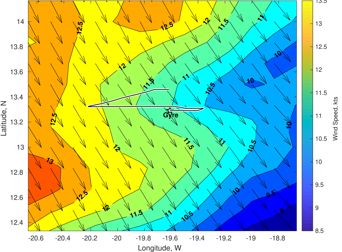
Winds (kts) for Gyre at 25-Jul-2025 09:00:00
