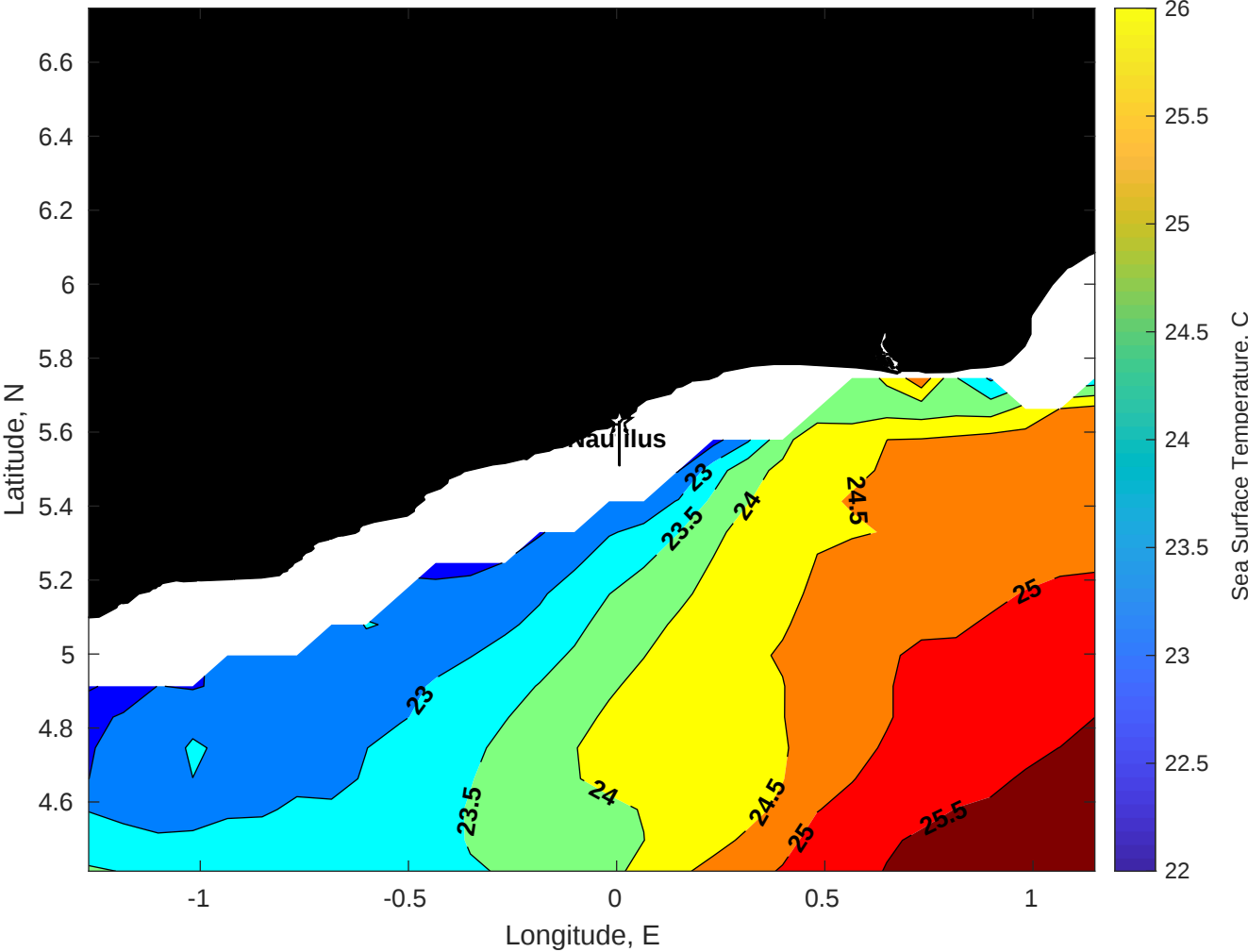
SST for Nautilus at 24-Jul-2025 00:00:00
