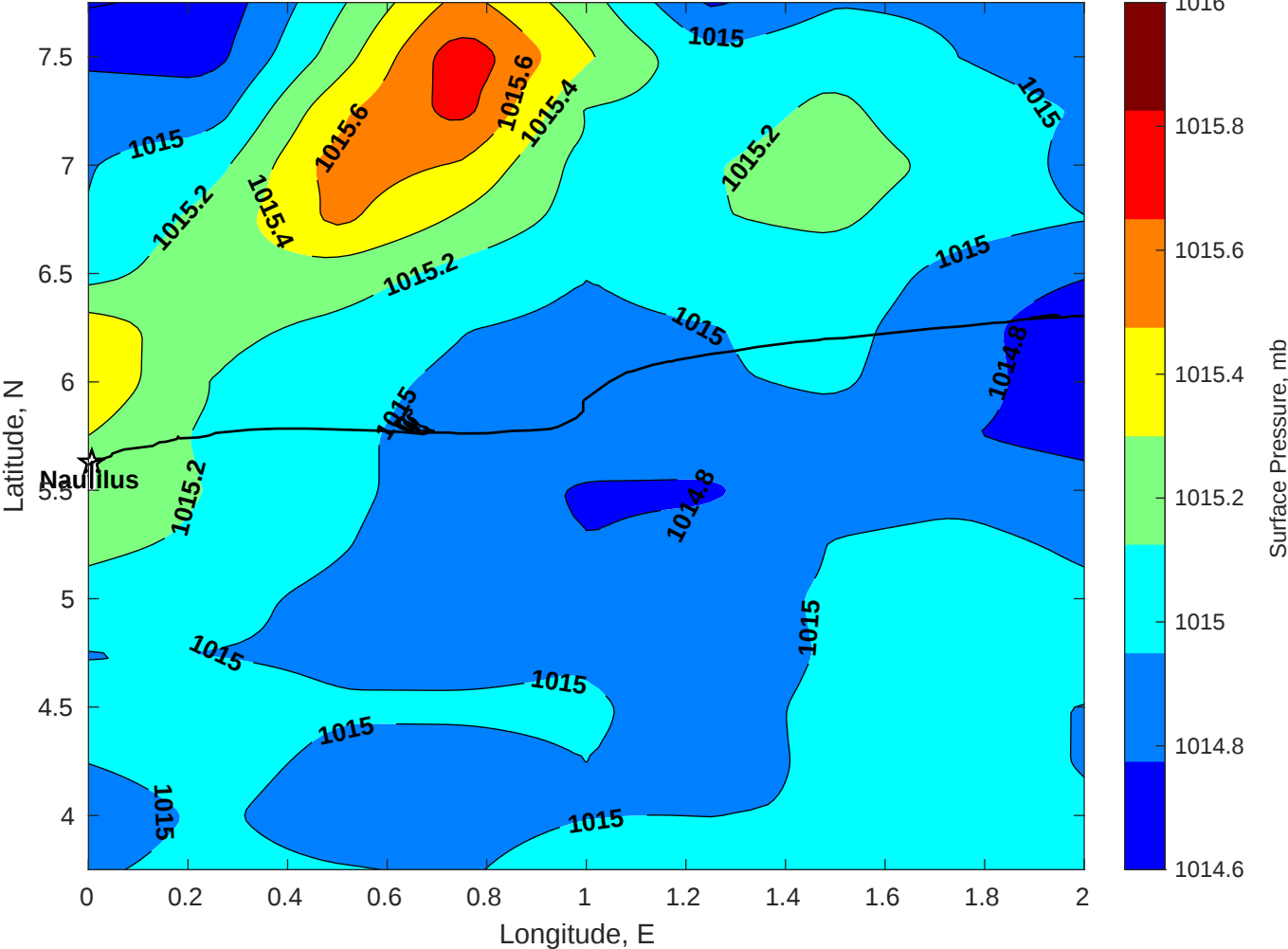
Surface Pressure (mb) for Nautilus at 25-Jul-2025 00:00:00
