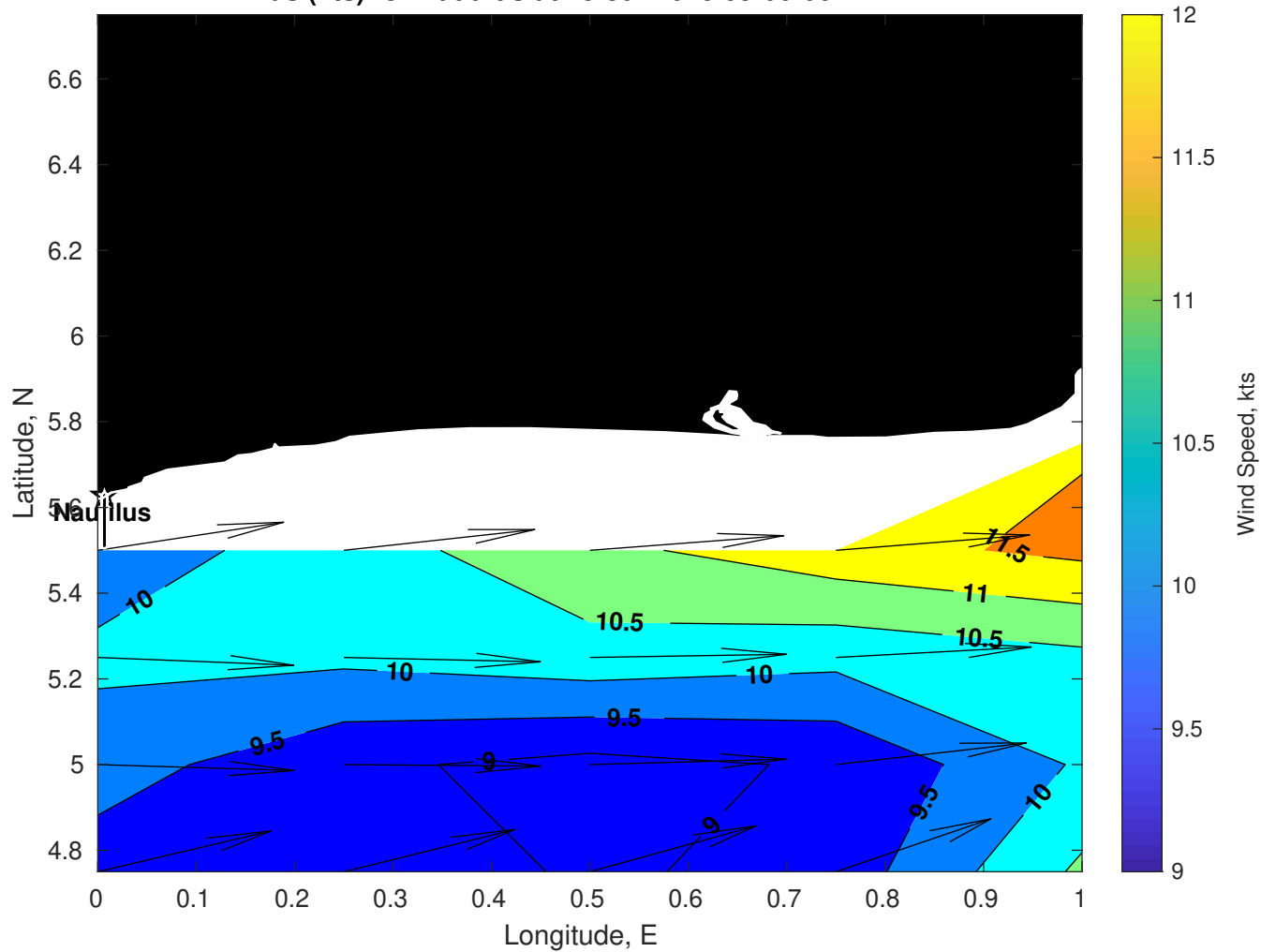
Winds (kts) for Nautilus at 25-Jul-2025 09:00:00
