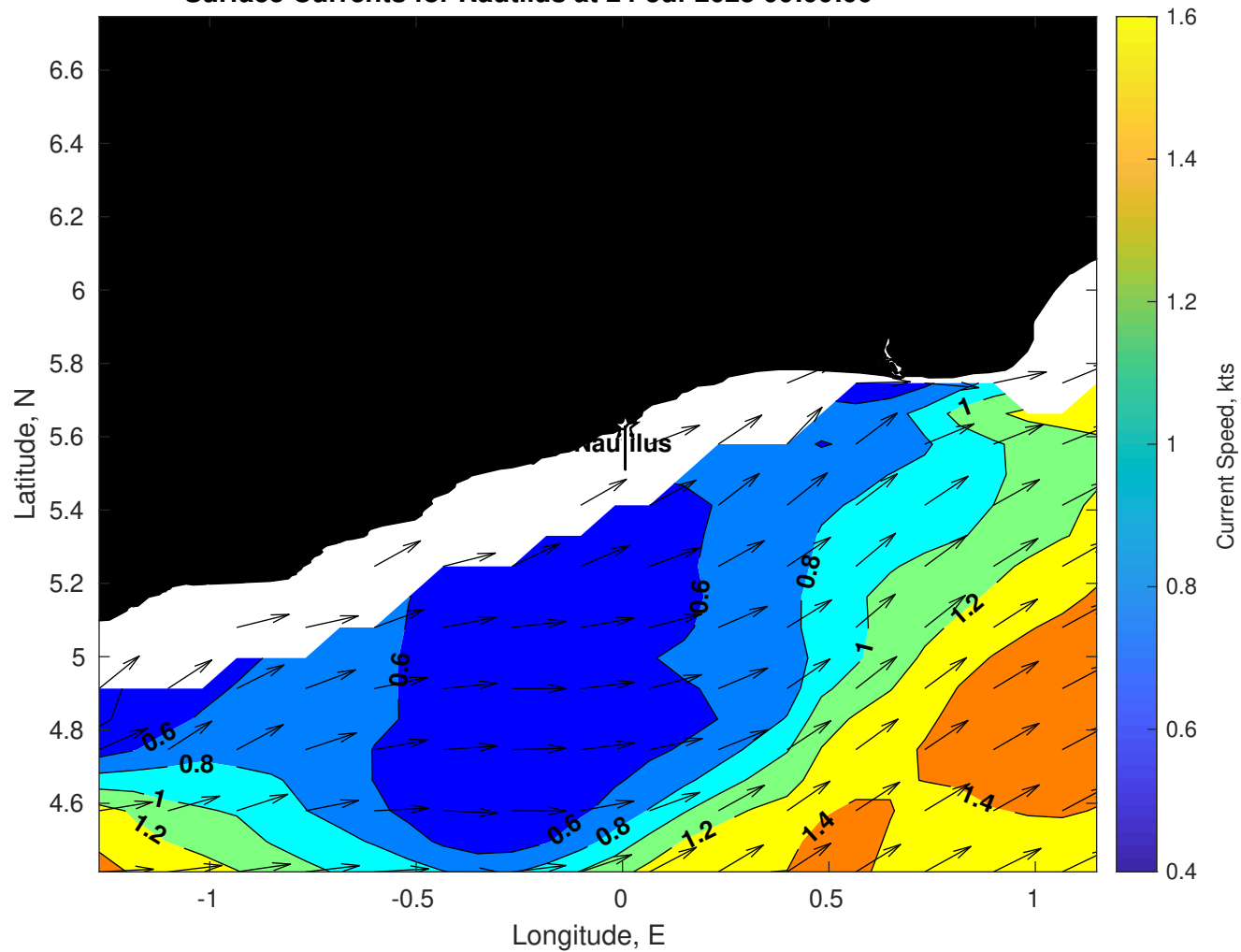
Surface Currents for Nautilus at 24-Jul-2025 00:00:00
