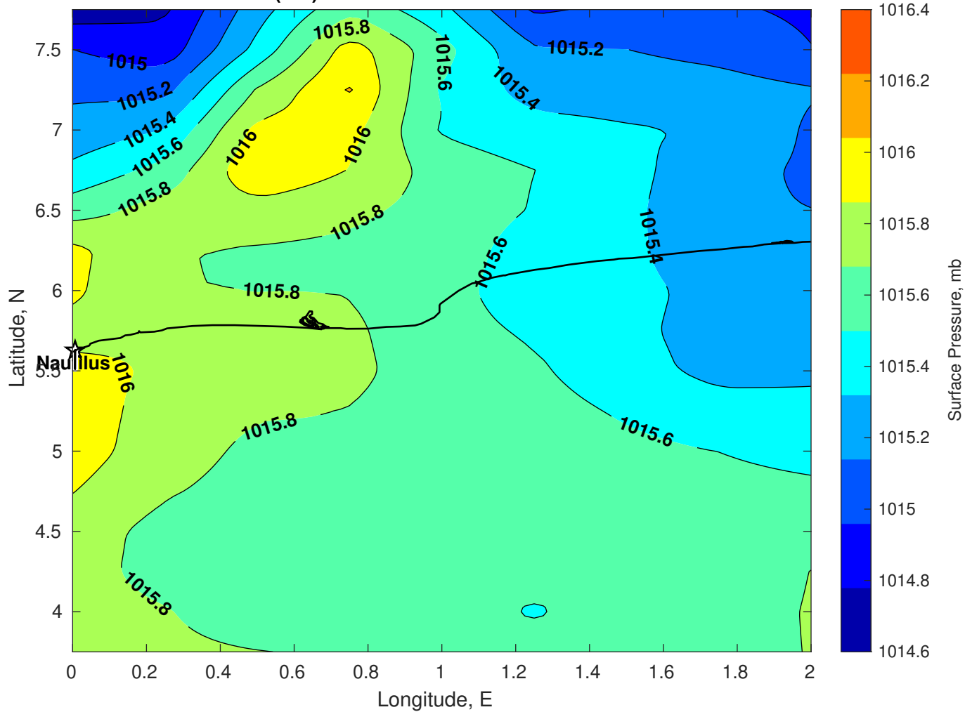
Surface Pressure (mb) for Nautilus at 26-Jul-2025 00:00:00
