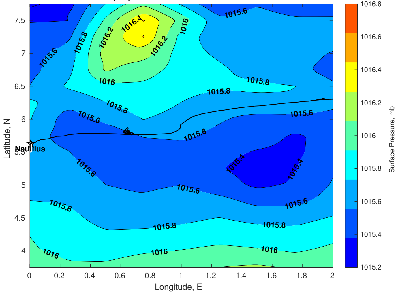
Surface Pressure (mb) for Nautilus at 27-Jul-2025 00:00:00
