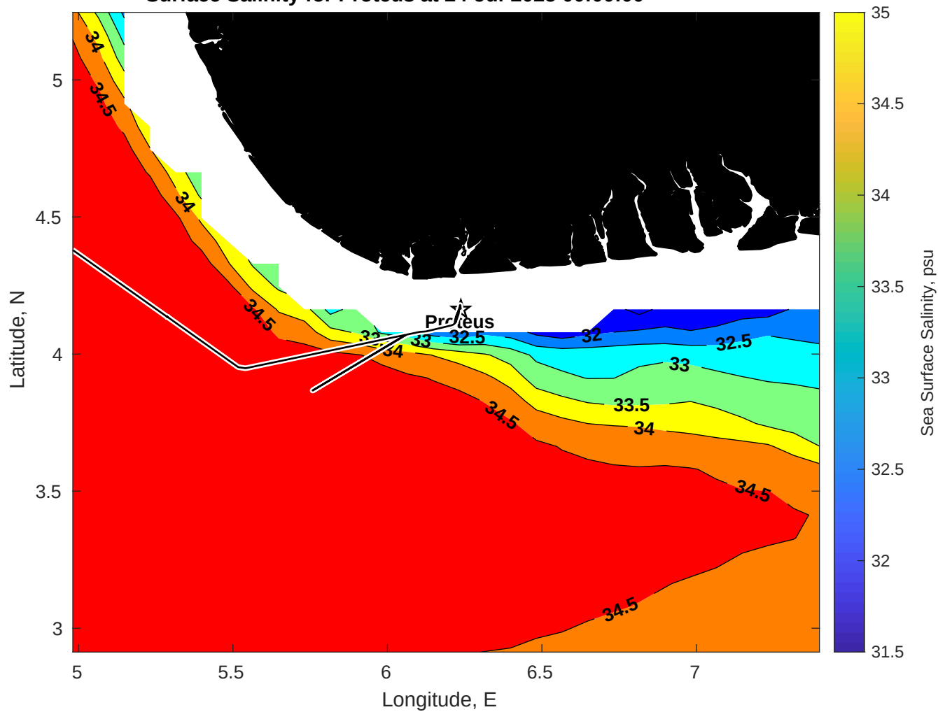
Surface Salinity for Proteus at 24-Jul-2025 00:00:00
