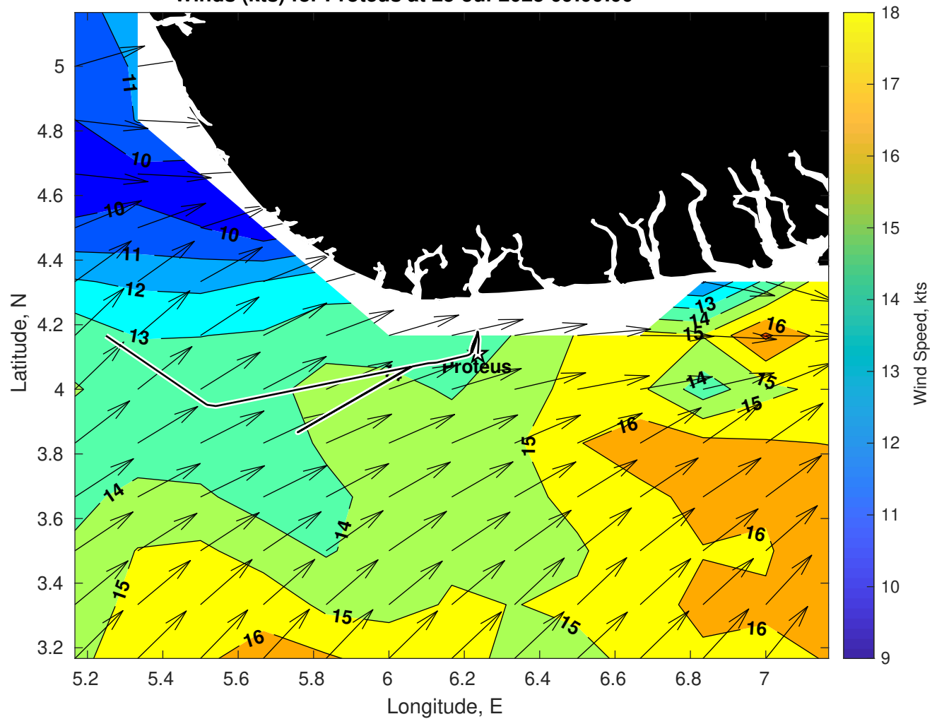
Winds (kts) for Proteus at 25-Jul-2025 09:00:00
