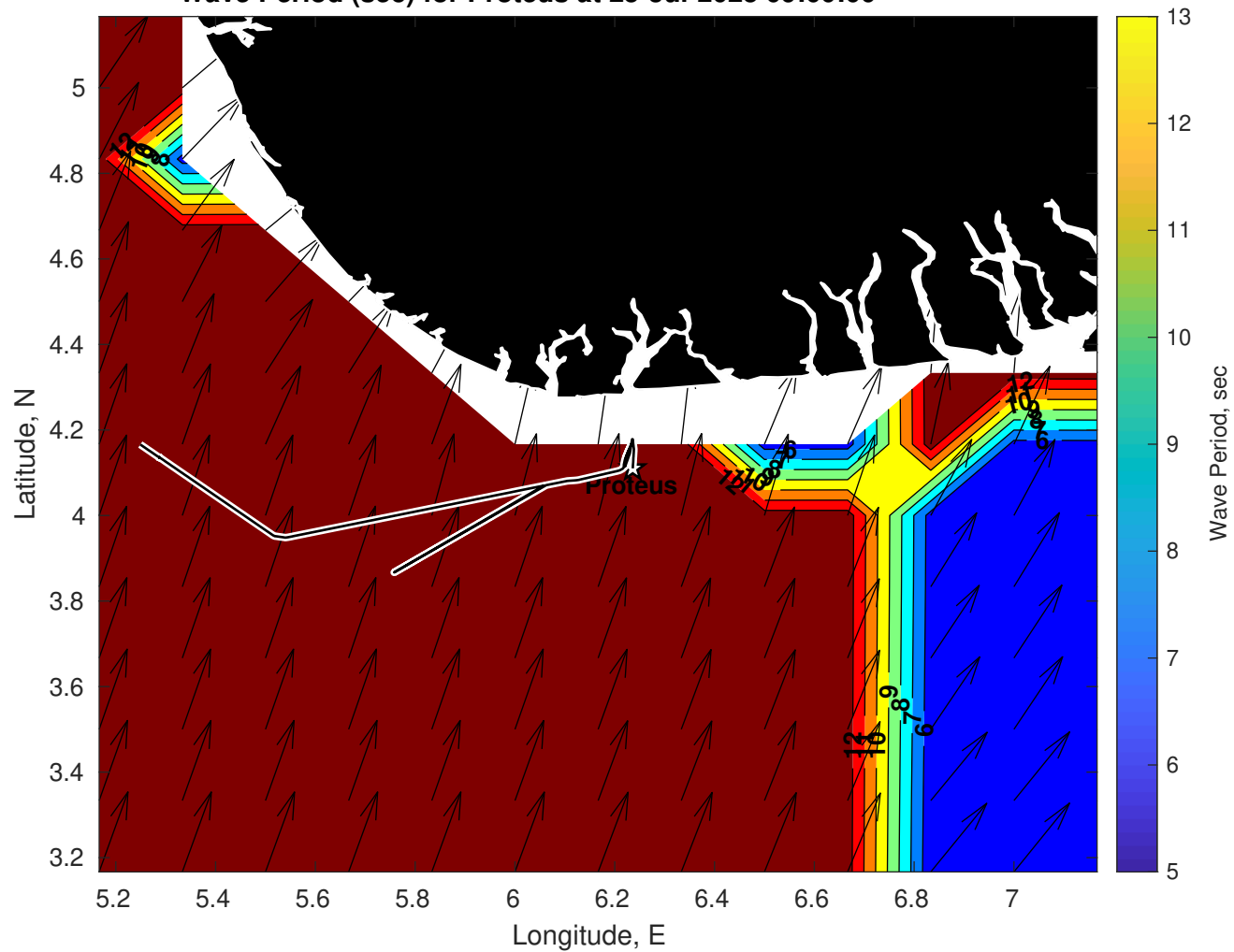
Wave Period (sec) for Proteus at 25-Jul-2025 09:00:00
