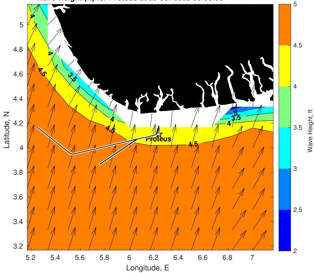
Wave Height (ft) for Proteus at 25-Jul-2025 09:00:00
