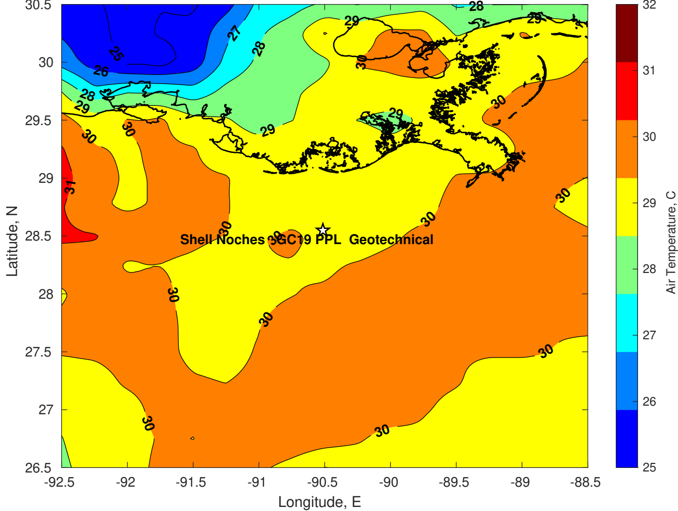
Air Temperature (C) for Shell Noches GC19 PPL Geotechnical at 25-Jul-2025
