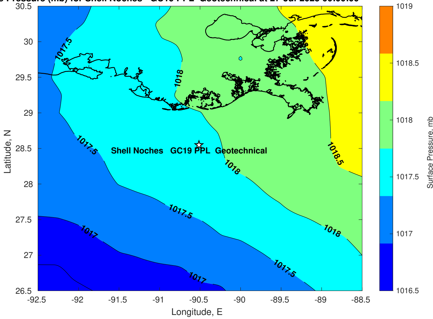
Surface Pressure (mb) for Shell Noches GC19 PPL Geotechnical at 27-Jul-2025 00:00:00
