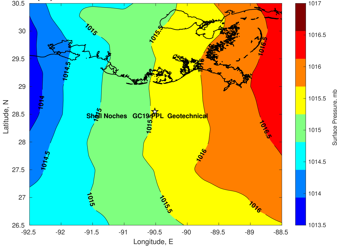
Surface Pressure (mb) for Shell Noches GC19 PPL Geotechnical at 26-Jul-2025 00:00:00
