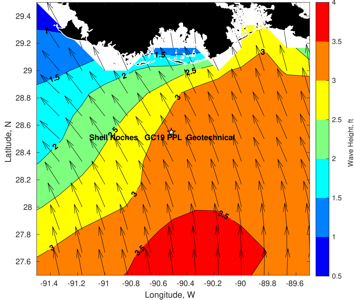
Wave Height (ft) for Shell Noches GC19 PPL Geotechnical at 25-Jul-2025 09:00:00
