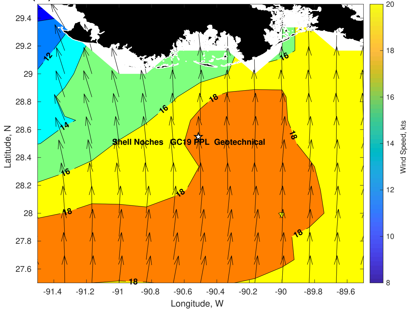
Winds (kts) for Shell Noches GC19 PPL Geotechnical at 25-Jul-2025 09:00:00
