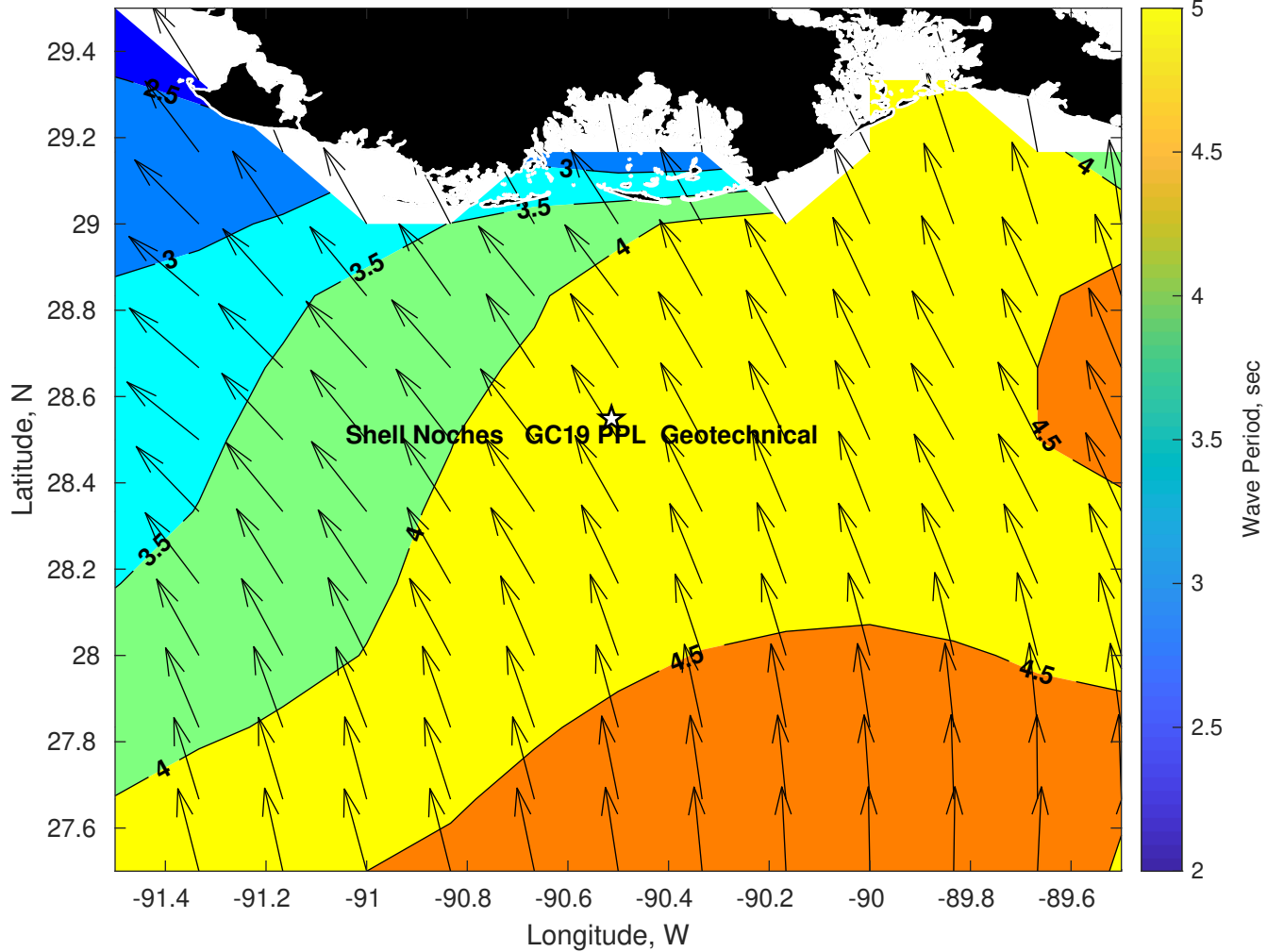
Wave Period (sec) for Shell Noches GC19 PPL Geotechnical at 25-Jul-2025 09:00:00
