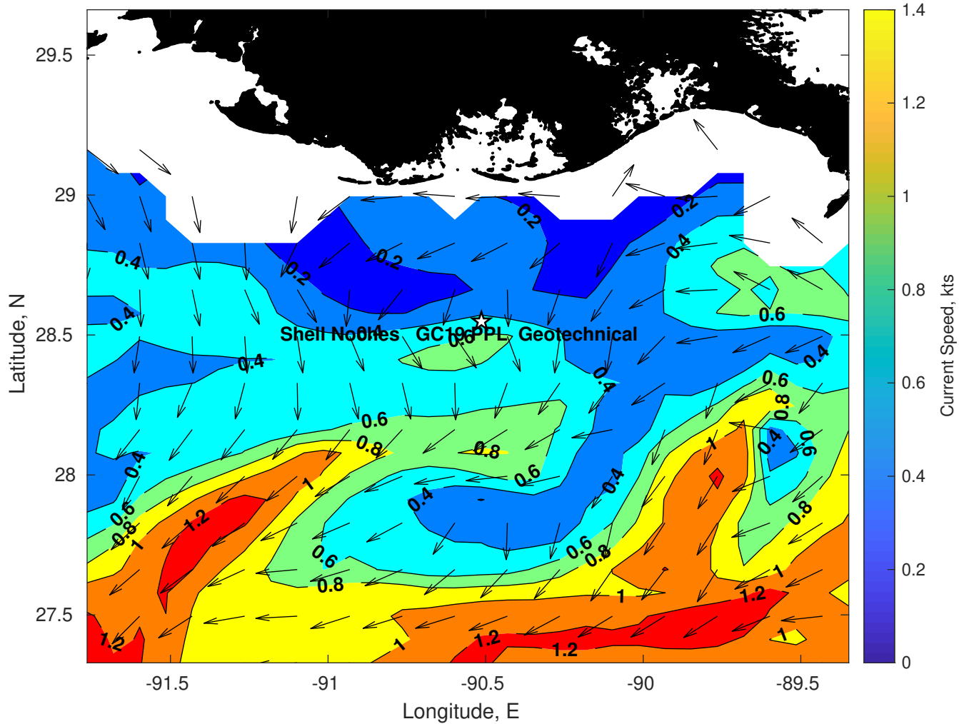
Surface Currents for Shell Noches GC19 PPL Geotechnical at 24-Jul-2025 00:00:00
