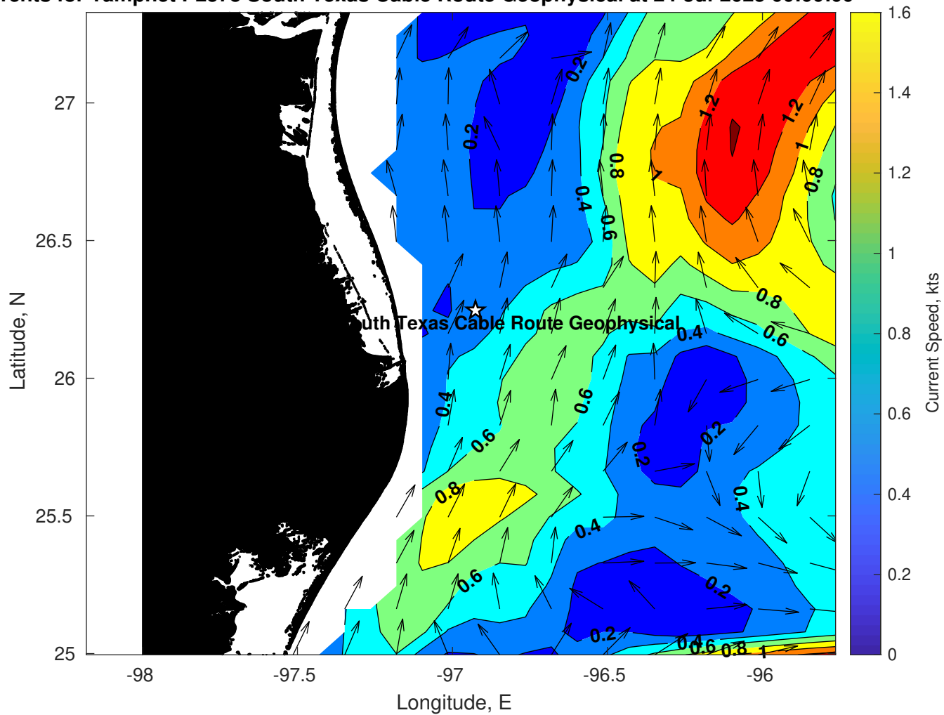
Surface Currents for Tampnet P2378 South Texas Cable Route Geophysical at 24-Jul-2025 00:00:00
