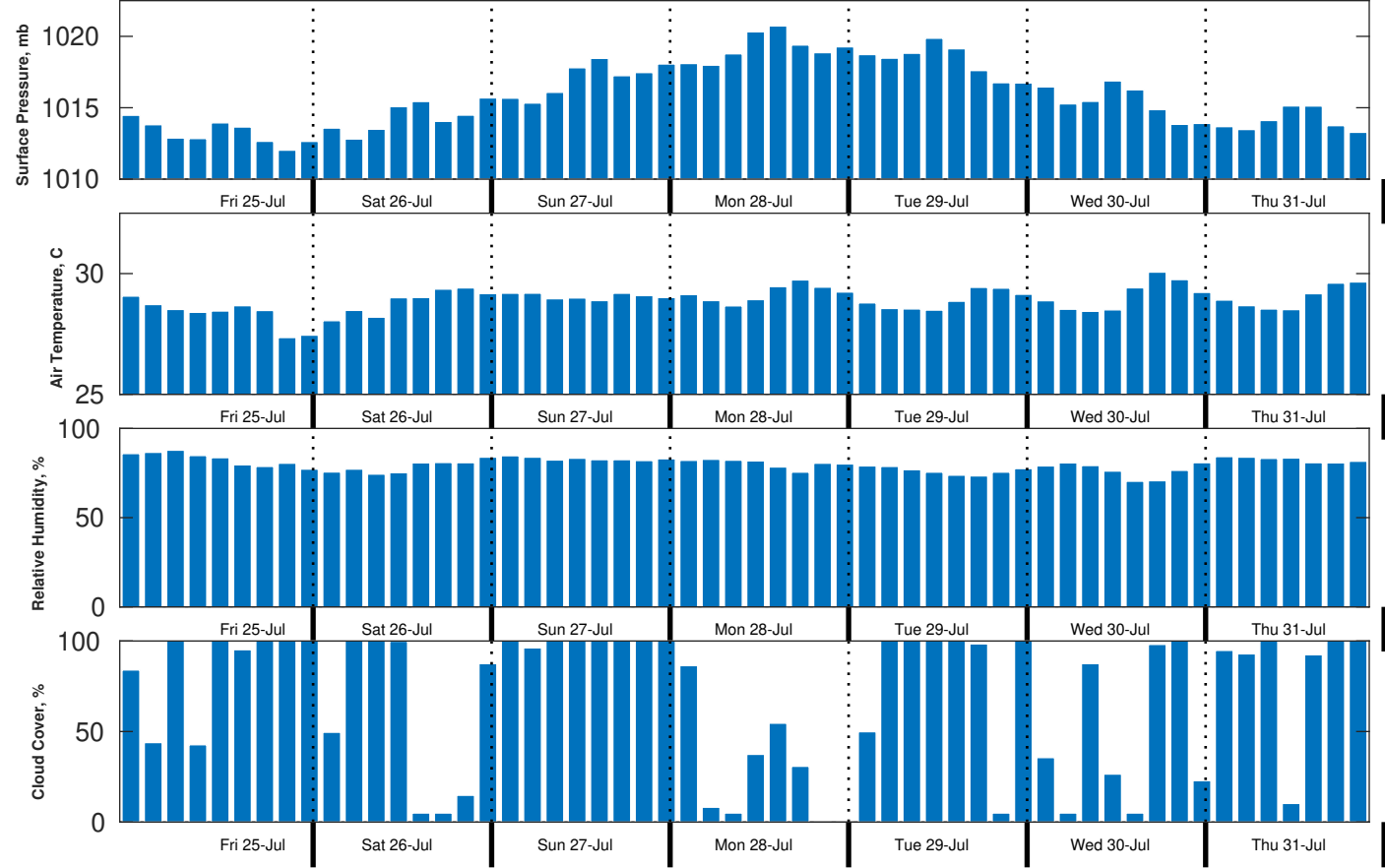
Met Forecast for Tampnet P2378 South Texas Cable Route Geophysical from 25-Jul-2025 00:00:00 to 01-Aug-2025 00:00:00
