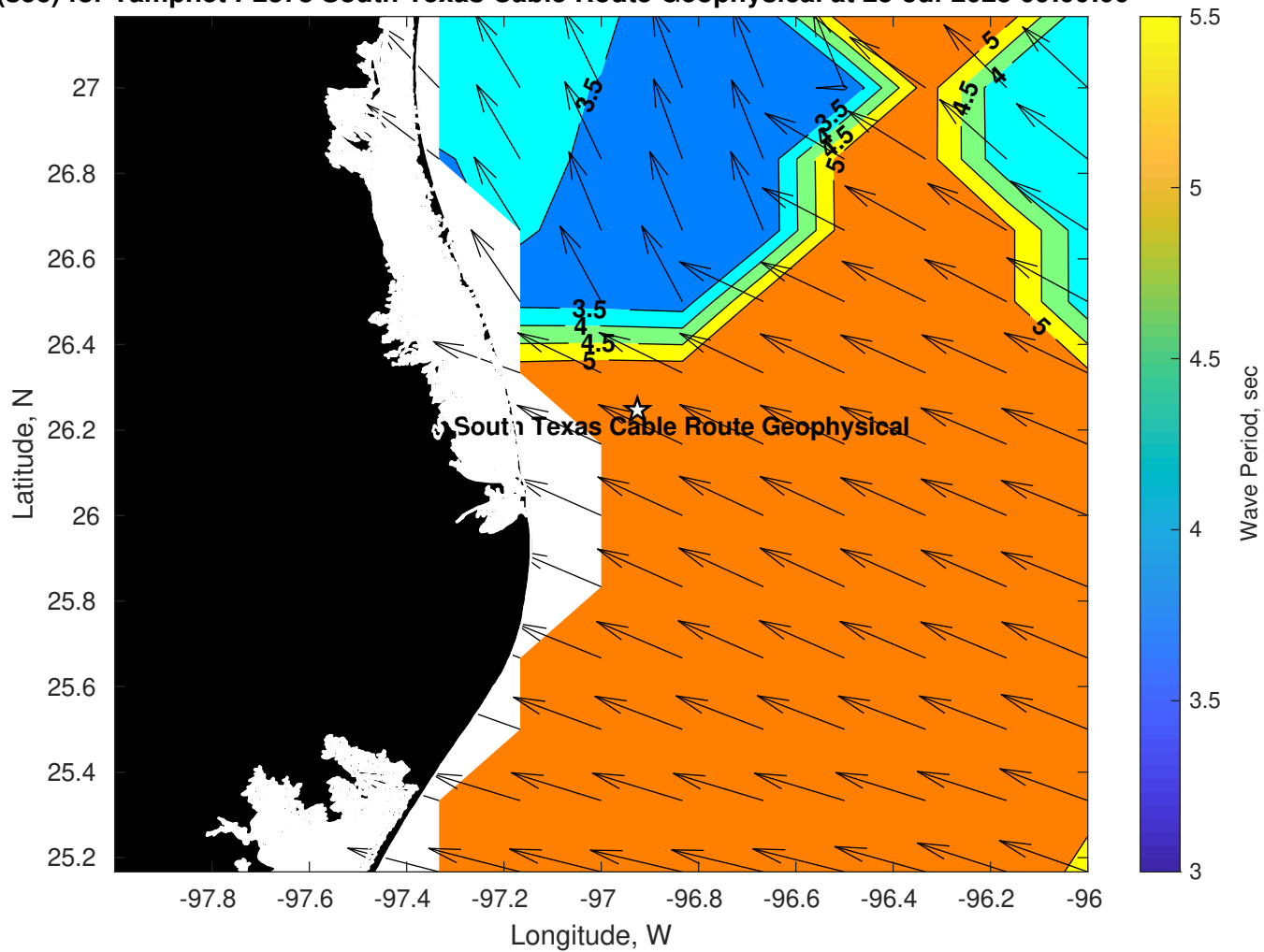
Wave Period (sec) for Tampnet P2378 South Texas Cable Route Geophysical at 25-Jul-2025 09:00:00
