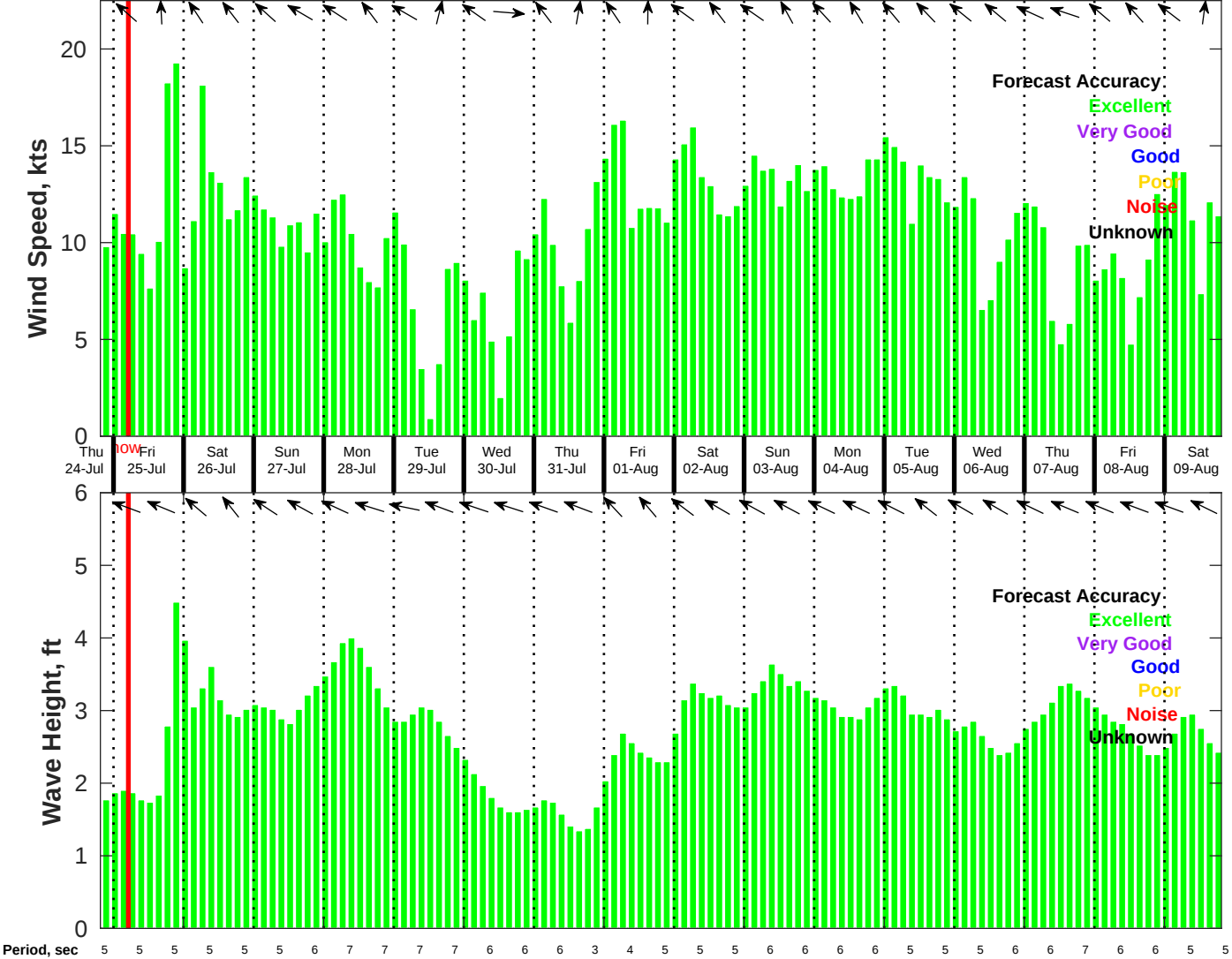
Wind & Wave Forecast for Tampnet P2378 South Texas Cable Route Geophysical from 24-Jul-2025 20:00:00 to 09-Aug-2025 20:00:00
