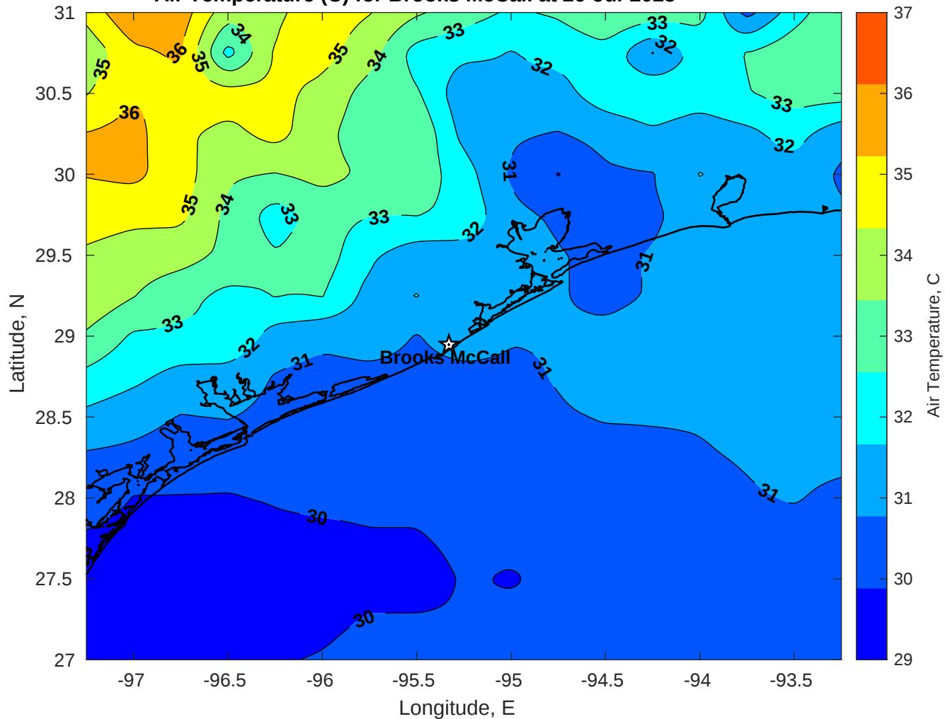
Air Temperature (C) for Brooks McCall at 26-Jul-2025
