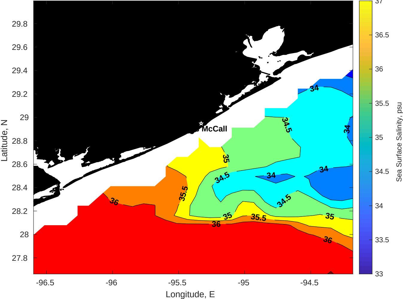
Surface Salinity for Brooks McCall at 25-Jul-2025 00:00:00
