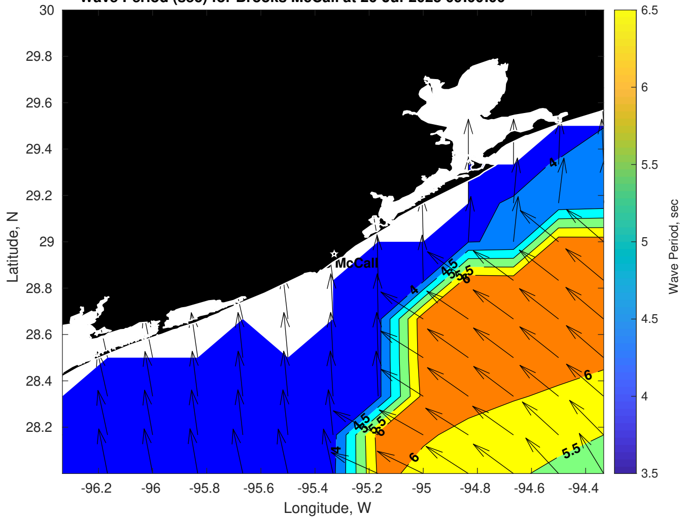
Wave Period (sec) for Brooks McCall at 26-Jul-2025 09:00:00
