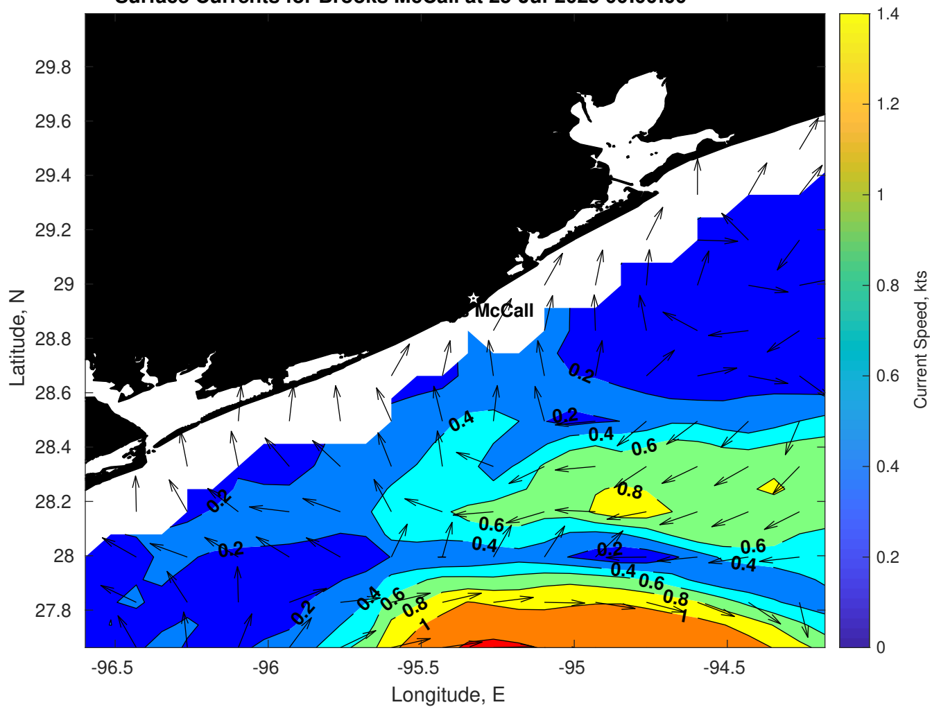
Surface Currents for Brooks McCall at 25-Jul-2025 00:00:00
