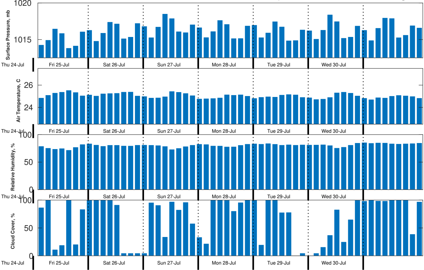
Met Forecast for CSA (ONHYM) PPL EBS - Cote d'Ivoire from 25-Jul-2025 00:00:00 to 01-Aug-2025 00:00:00
