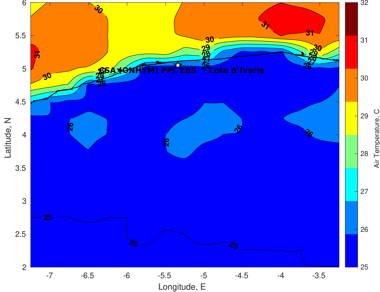
Air Temperature (C) for CSA (ONHYM) PPL EBS - Cote d'Ivoire at 25-Jul-2025
