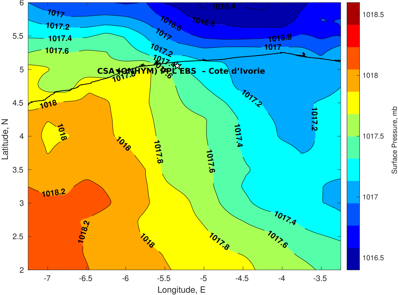
Surface Pressure (mb) for CSA (ONHYM) PPL EBS - Cote d'Ivoire at 27-Jul-2025 12:00:00
