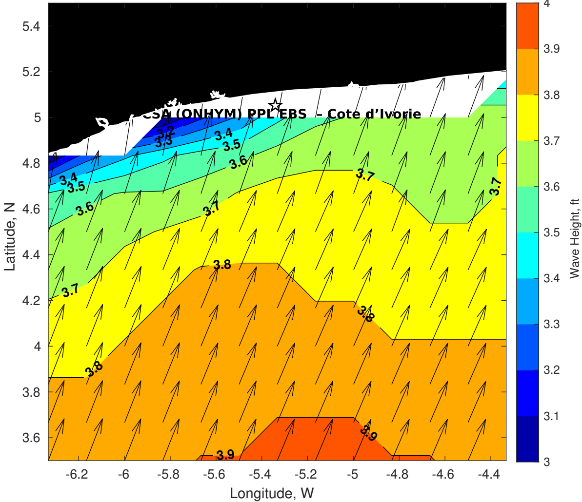
Wave Height (ft) for CSA (ONHYM) PPL EBS - Cote d'Ivoire at 25-Jul-2025 21:00:00
