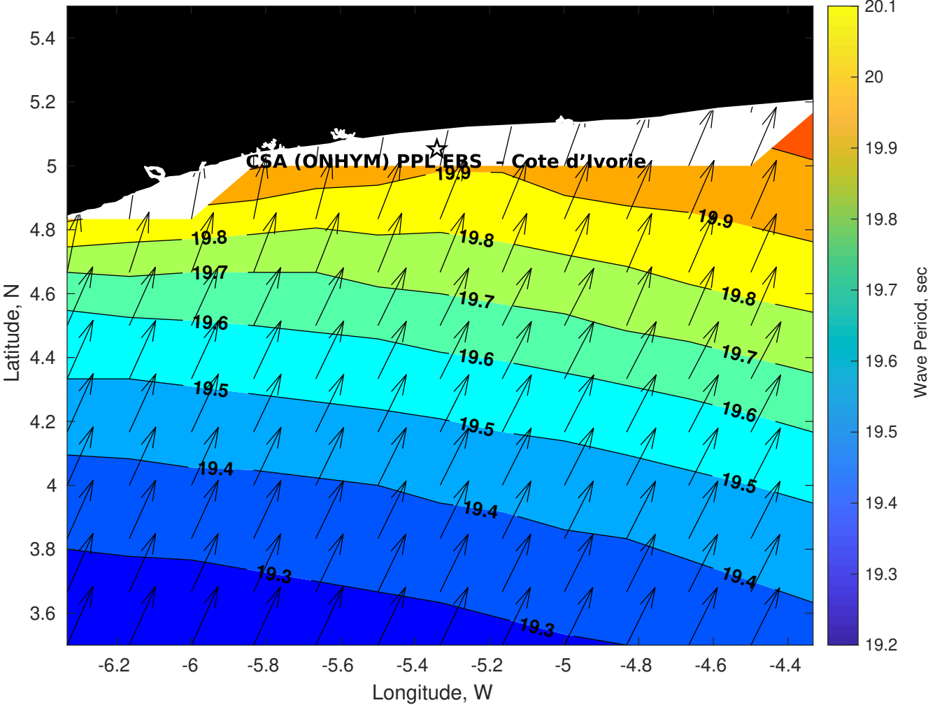
Wave Period (sec) for CSA (ONHYM) PPL EBS - Cote d'Ivoire at 25-Jul-2025 21:00:00
