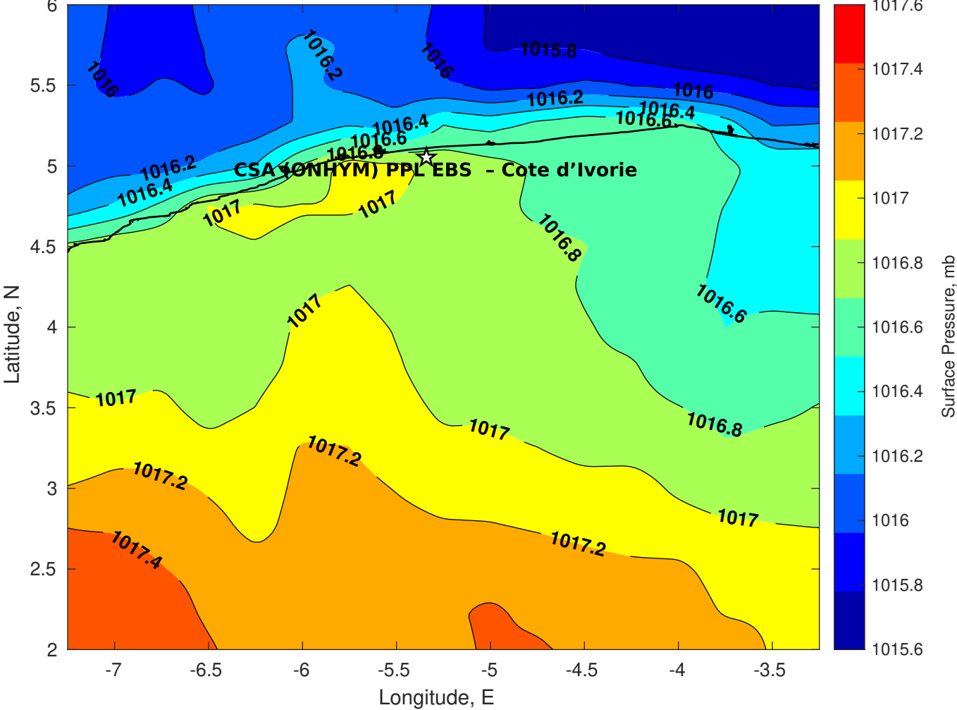
Surface Pressure (mb) for CSA (ONHYM) PPL EBS - Cote d'Ivoire at 26-Jul-2025 12:00:00
