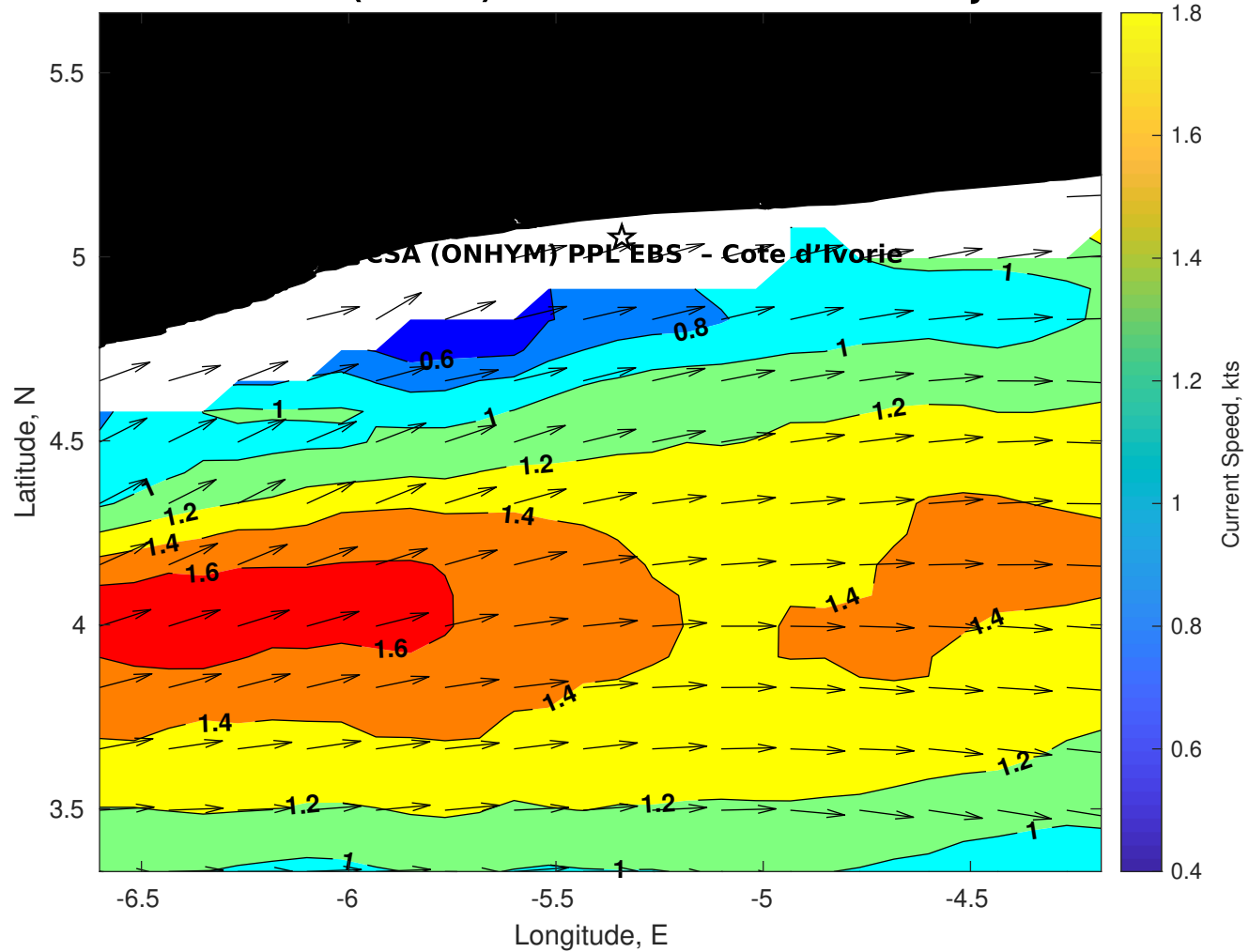
Surface Currents for CSA (ONHYM) PPL EBS - Cote d'Ivoire at 25-Jul-2025 00:00:00
