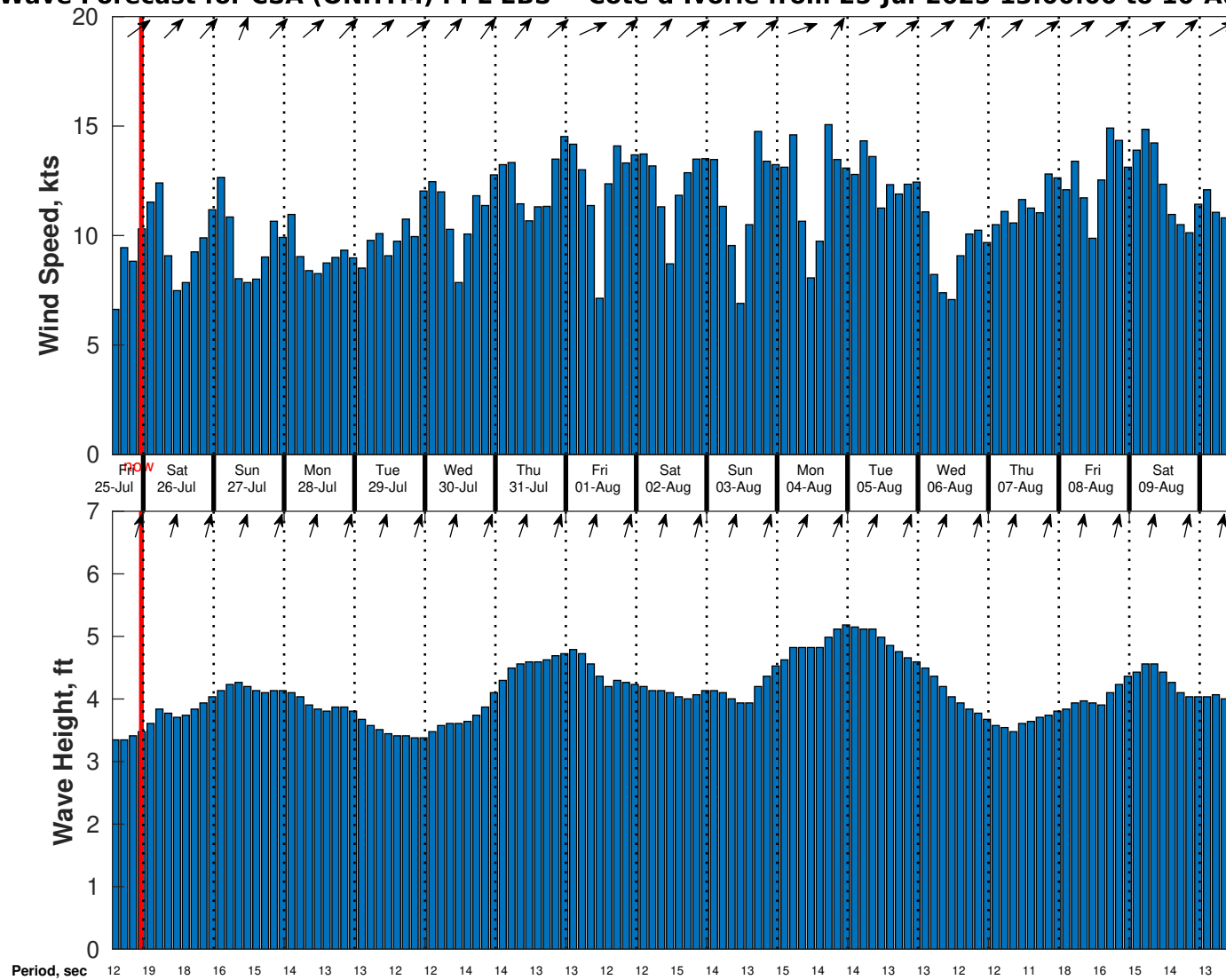
Wind & Wave Forecast for CSA (ONHYM) PPL EBS - Cote d'Ivoire from 25-Jul-2025 13:00:00 to 10-Aug-2025 13:00:00
