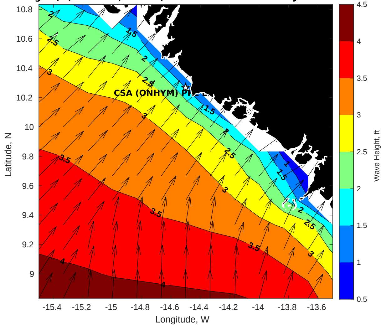
Wave Height (ft) for CSA (ONHYM) PPL EBS - Guinea at 25-Jul-2025 21:00:00
