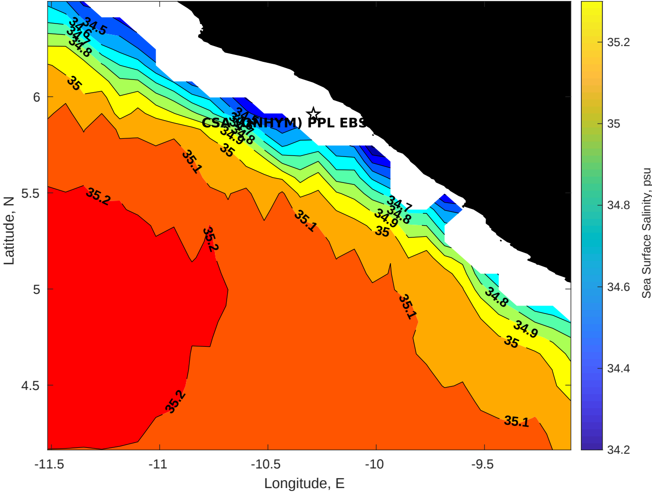
Surface Salinity for CSA (ONHYM) PPL EBS - Liberia at 25-Jul-2025 00:00:00
