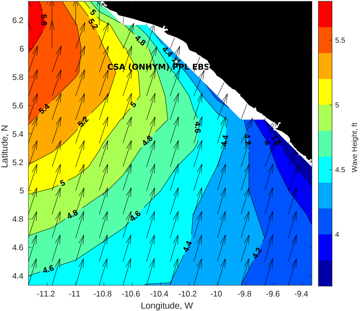
Wave Height (ft) for CSA (ONHYM) PPL EBS - Liberia at 25-Jul-2025 21:00:00
