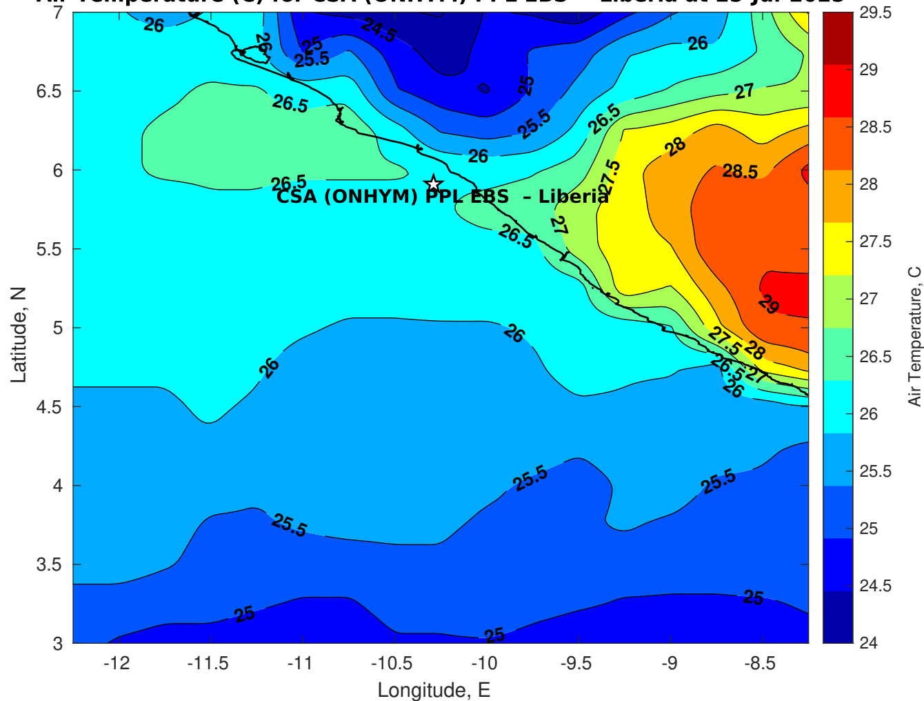
Air Temperature (C) for CSA (ONHYM) PPL EBS - Liberia at 25-Jul-2025
