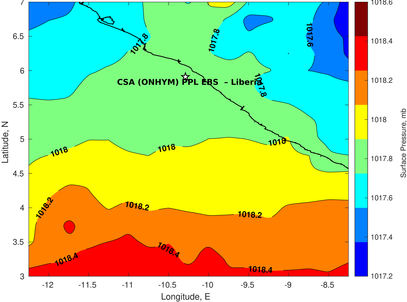
Surface Pressure (mb) for CSA (ONHYM) PPL EBS - Liberia at 27-Jul-2025 12:00:00
