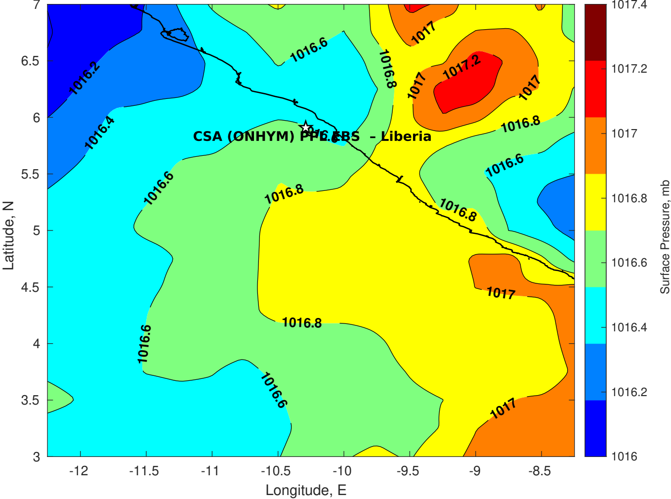
Surface Pressure (mb) for CSA (ONHYM) PPL EBS - Liberia at 26-Jul-2025 12:00:00
