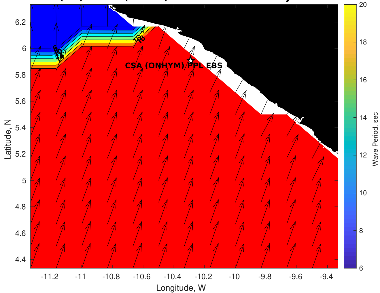
Wave Period (sec) for CSA (ONHYM) PPL EBS - Liberia at 25-Jul-2025 21:00:00
