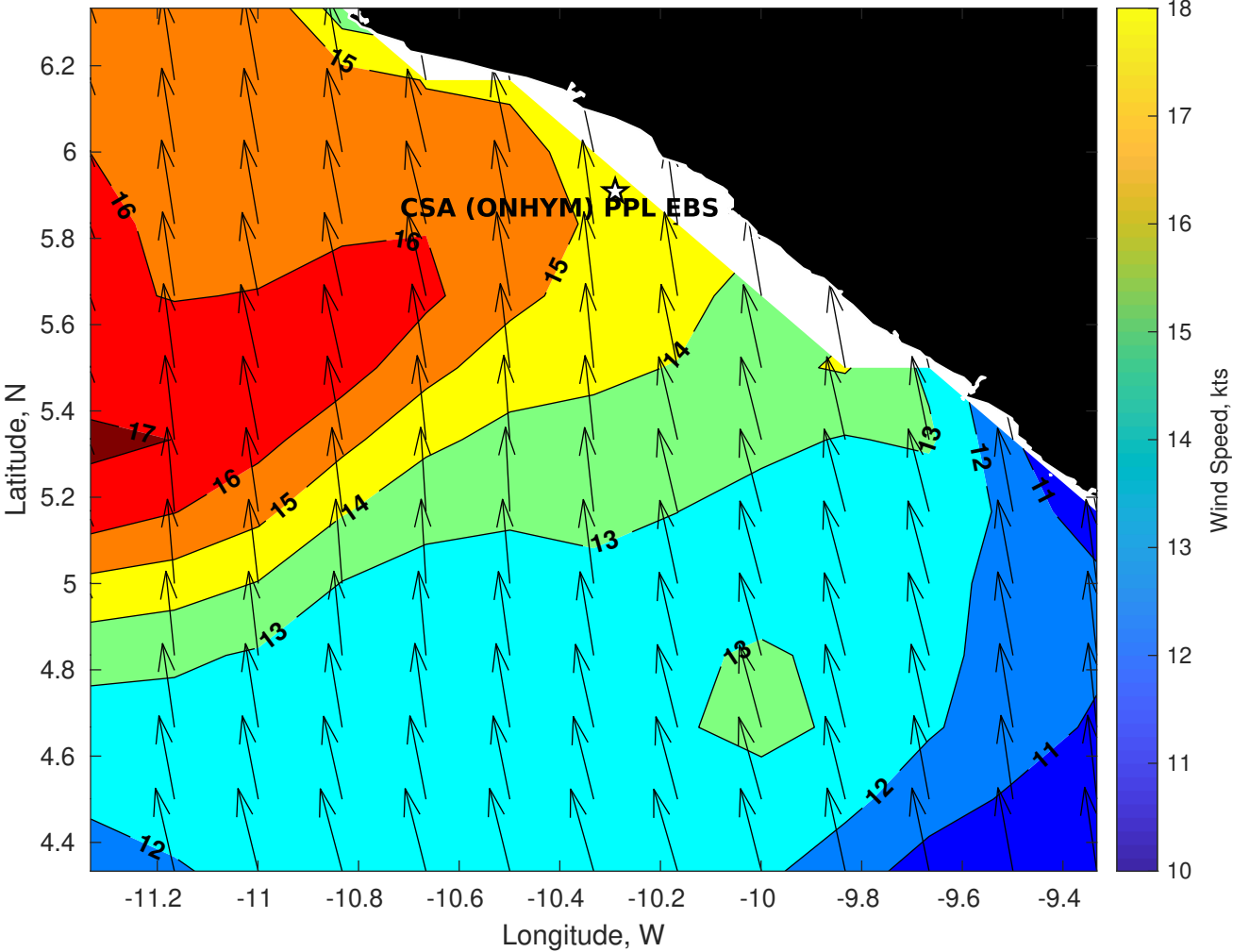
Winds (kts) for CSA (ONHYM) PPL EBS - Liberia at 25-Jul-2025 21:00:00
