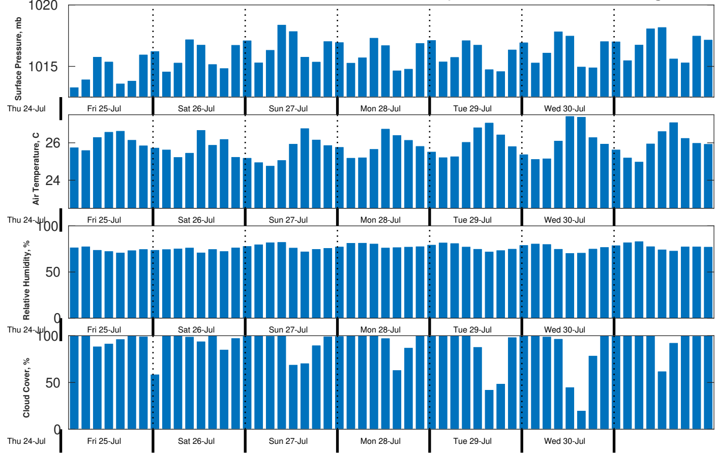
Met Forecast for CSA (ONHYM) PPL EBS - Liberia from 25-Jul-2025 00:00:00 to 01-Aug-2025 00:00:00
