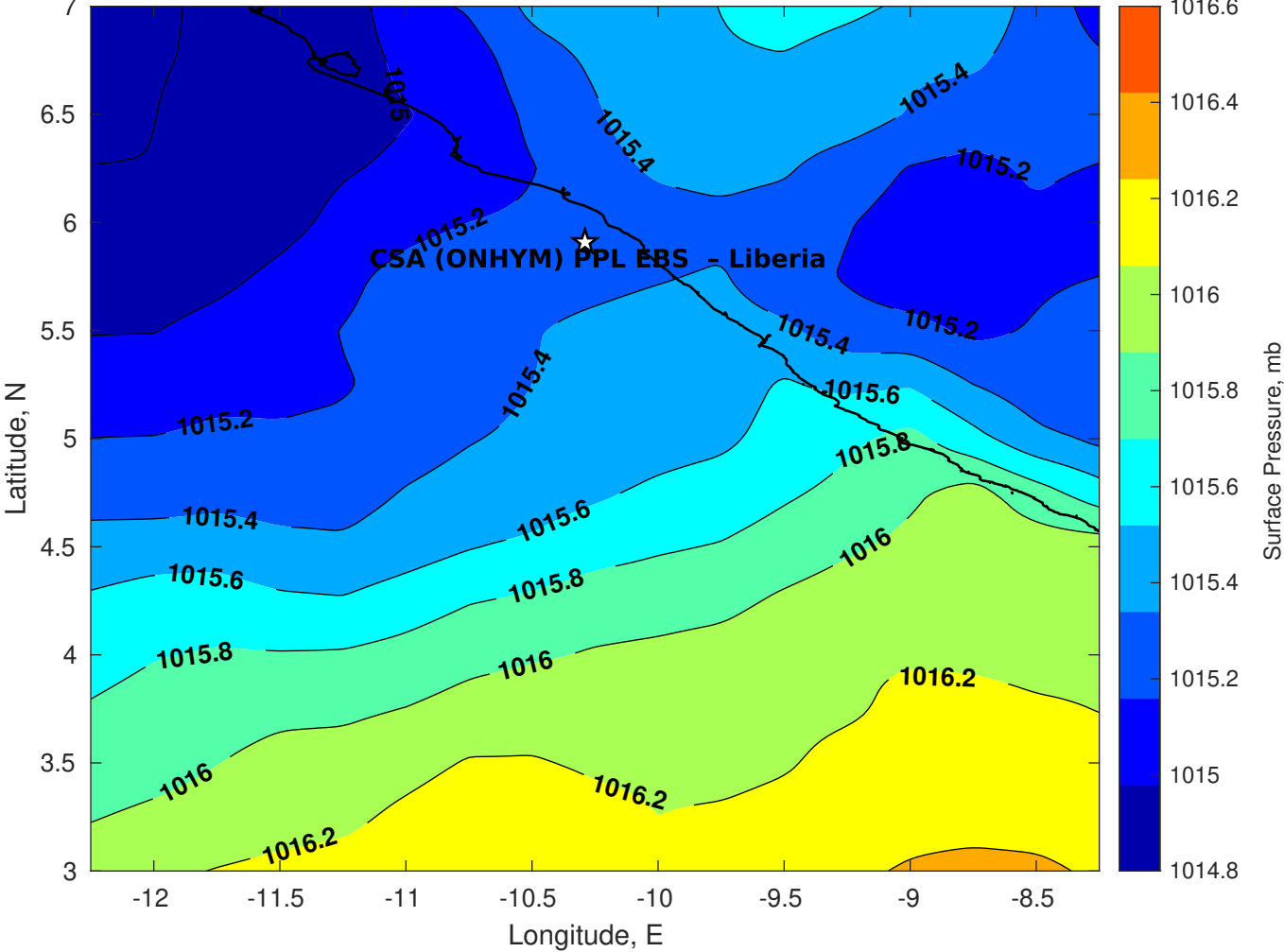
Surface Pressure (mb) for CSA (ONHYM) PPL EBS - Liberia at 26-Jul-2025 00:00:00
