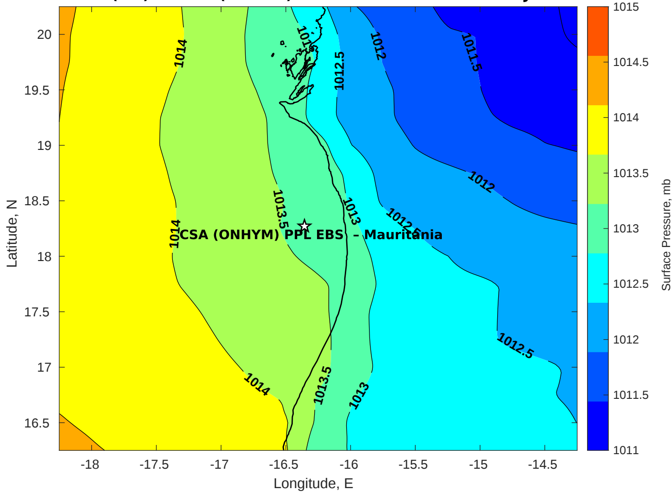
Surface Pressure (mb) for CSA (ONHYM) PPL EBS - Mauritania at 26-Jul-2025 12:00:00
