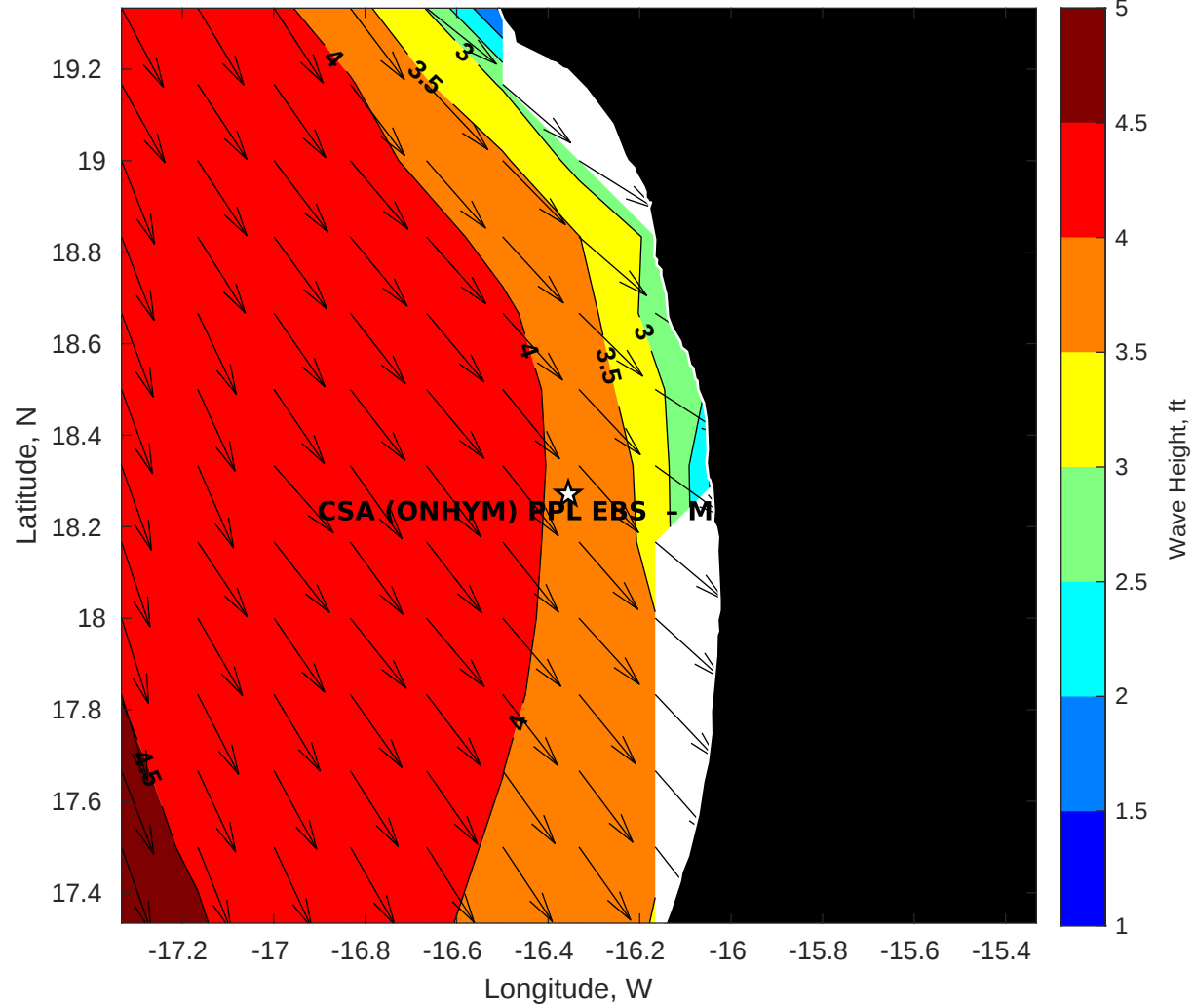
Wave Height (ft) for CSA (ONHYM) PPL EBS - Mauritania at 25-Jul-2025 21:00:00
