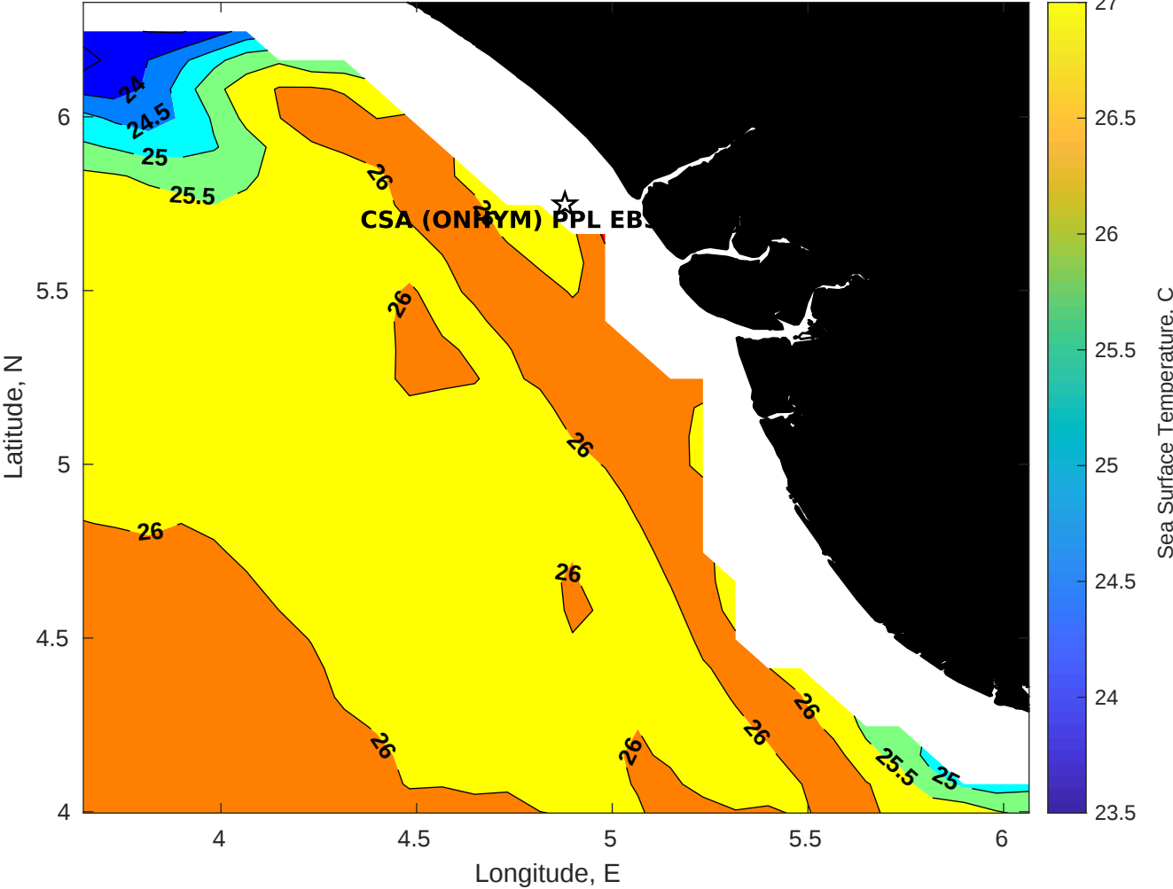
SST for CSA (ONHYM) PPL EBS - Nigeria at 25-Jul-2025 00:00:00
