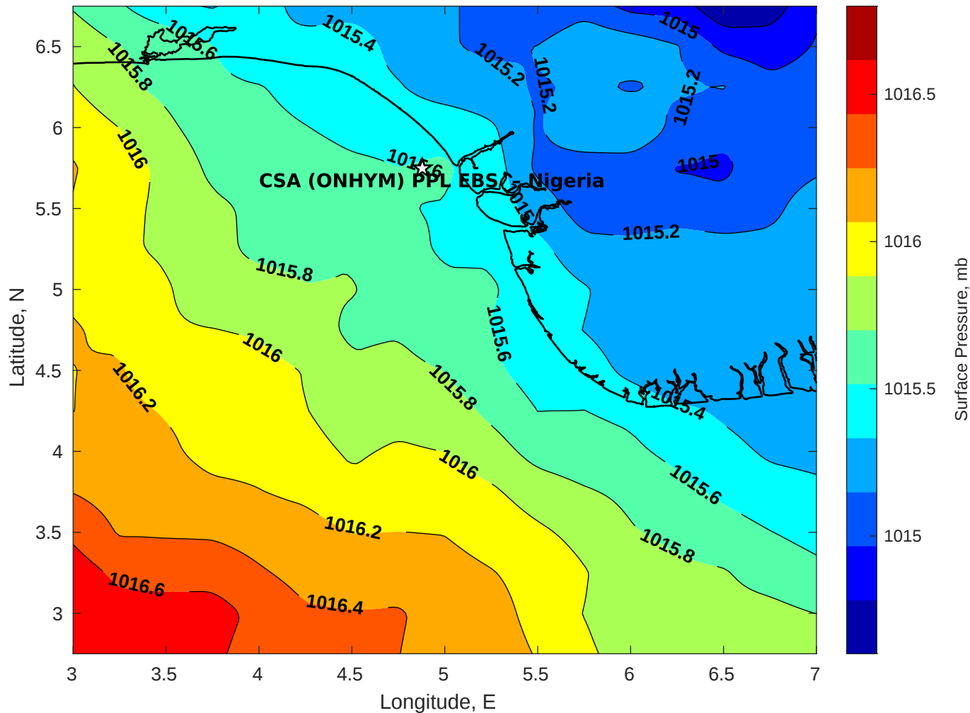
Surface Pressure (mb) for CSA (ONHYM) PPL EBS - Nigeria at 27-Jul-2025 12:00:00
