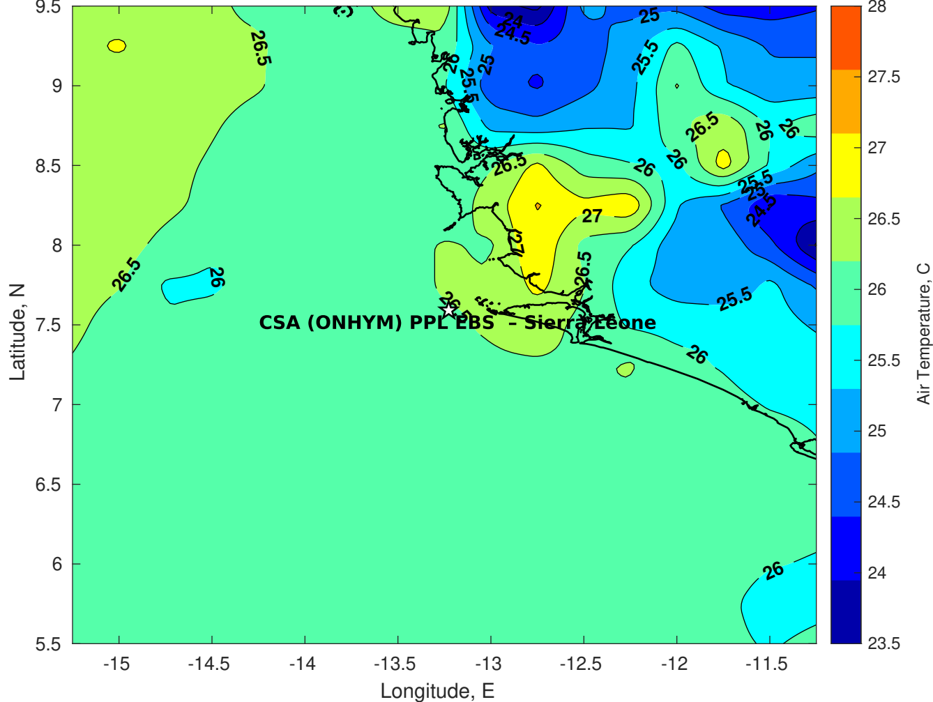
Air Temperature (C) for CSA (ONHYM) PPL EBS - Sierra Leone at 25-Jul-2025
