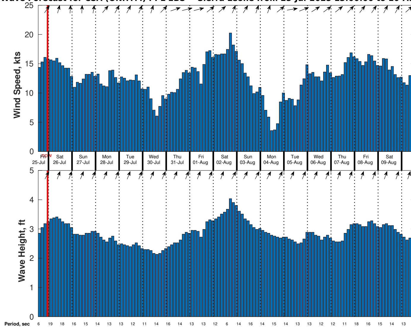
Wind & Wave Forecast for CSA (ONHYM) PPL EBS - Sierra Leone from 25-Jul-2025 13:00:00 to 10-Aug-2025 13:00:00
