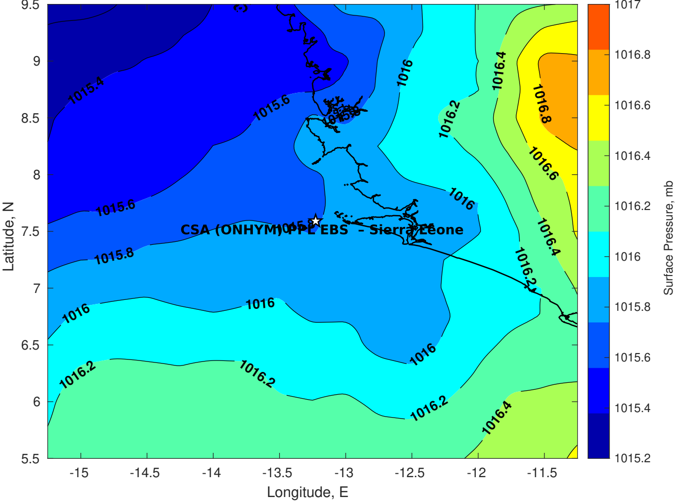
Surface Pressure (mb) for CSA (ONHYM) PPL EBS - Sierra Leone at 26-Jul-2025 12:00:00
