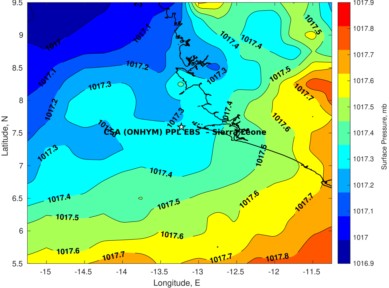
Surface Pressure (mb) for CSA (ONHYM) PPL EBS - Sierra Leone at 27-Jul-2025 12:00:00
