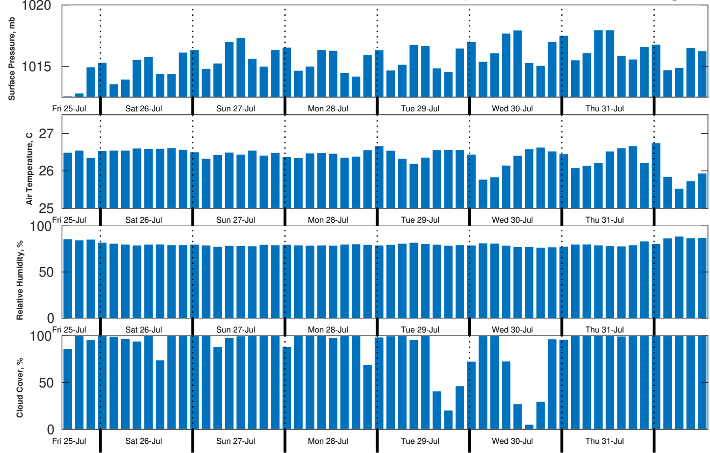
Met Forecast for CSA (ONHYM) PPL EBS - Sierra Leone from 25-Jul-2025 12:00:00 to 01-Aug-2025 12:00:00
