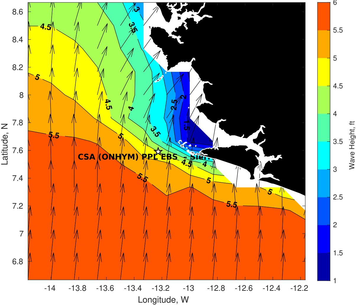
Wave Height (ft) for CSA (ONHYM) PPL EBS - Sierra Leone at 25-Jul-2025 21:00:00
