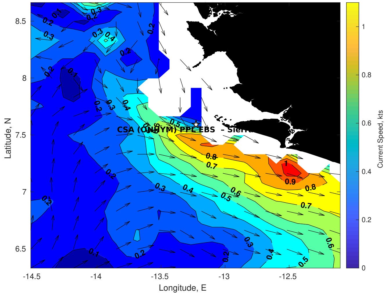
Surface Currents for CSA (ONHYM) PPL EBS - Sierra Leone at 25-Jul-2025 00:00:00
