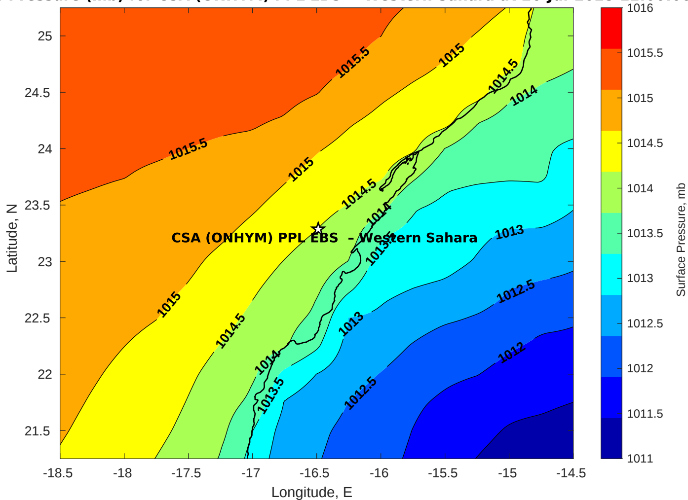
Surface Pressure (mb) for CSA (ONHYM) PPL EBS - Western Sahara at 26-Jul-2025 12:00:00
