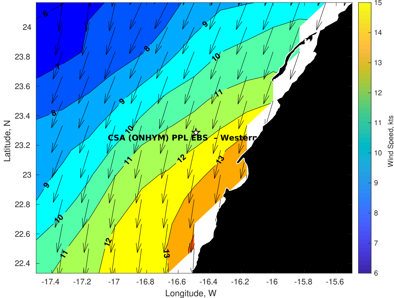
Winds (kts) for CSA (ONHYM) PPL EBS - Western Sahara at 25-Jul-2025 21:00:00
