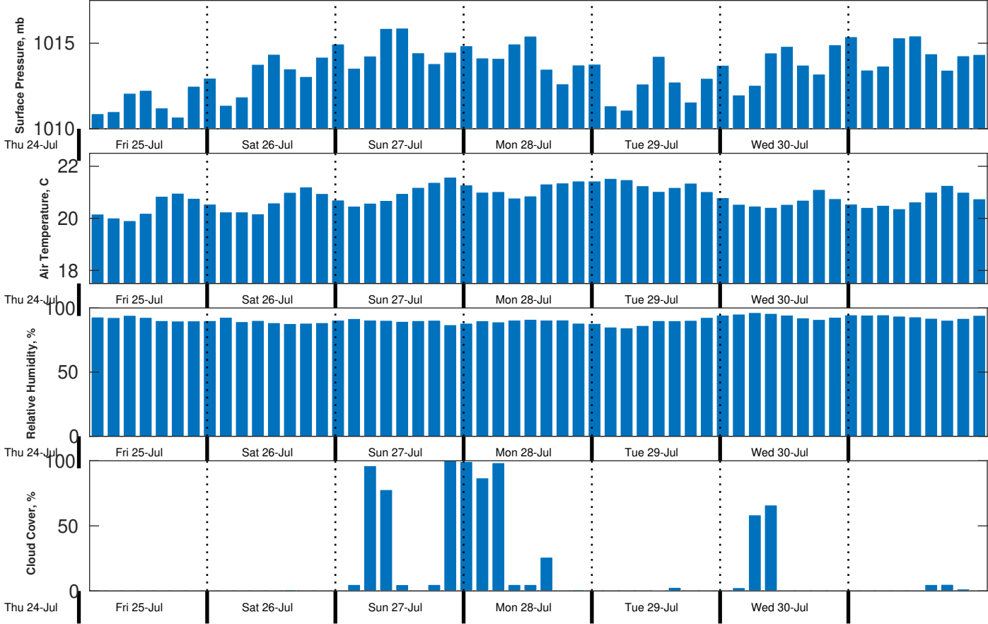
Met Forecast for CSA (ONHYM) PPL EBS - Western Sahara from 25-Jul-2025 00:00:00 to 01-Aug-2025 00:00:00
