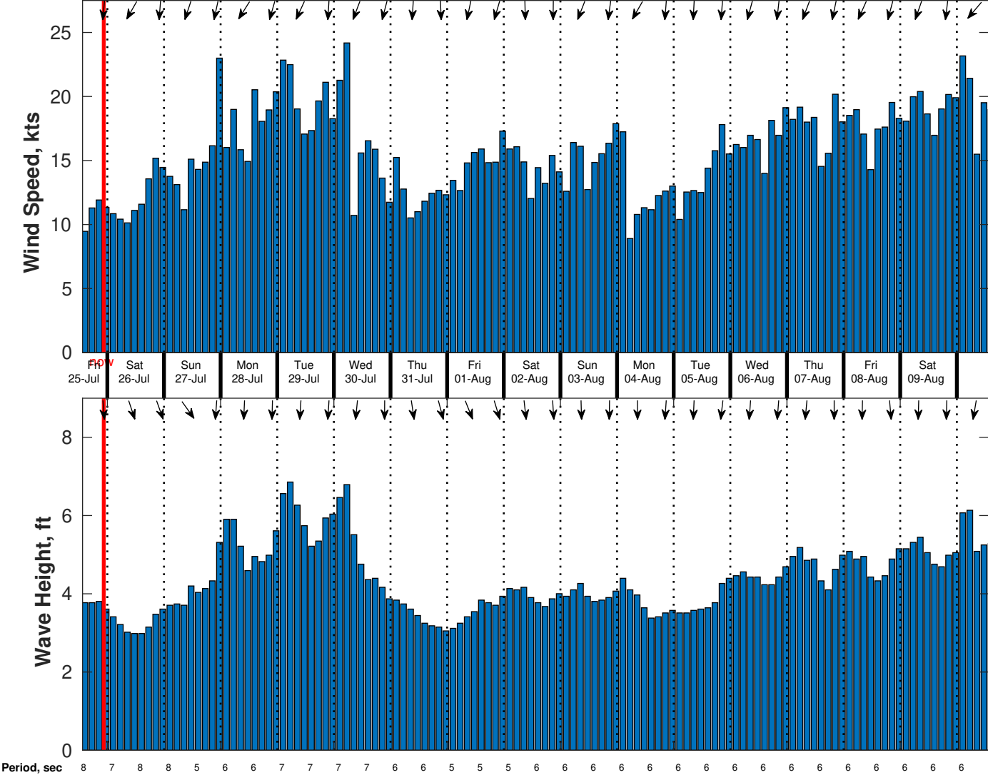
Wind & Wave Forecast for CSA (ONHYM) PPL EBS - Western Sahara from 25-Jul-2025 13:00:00 to 10-Aug-2025 13:00:00
