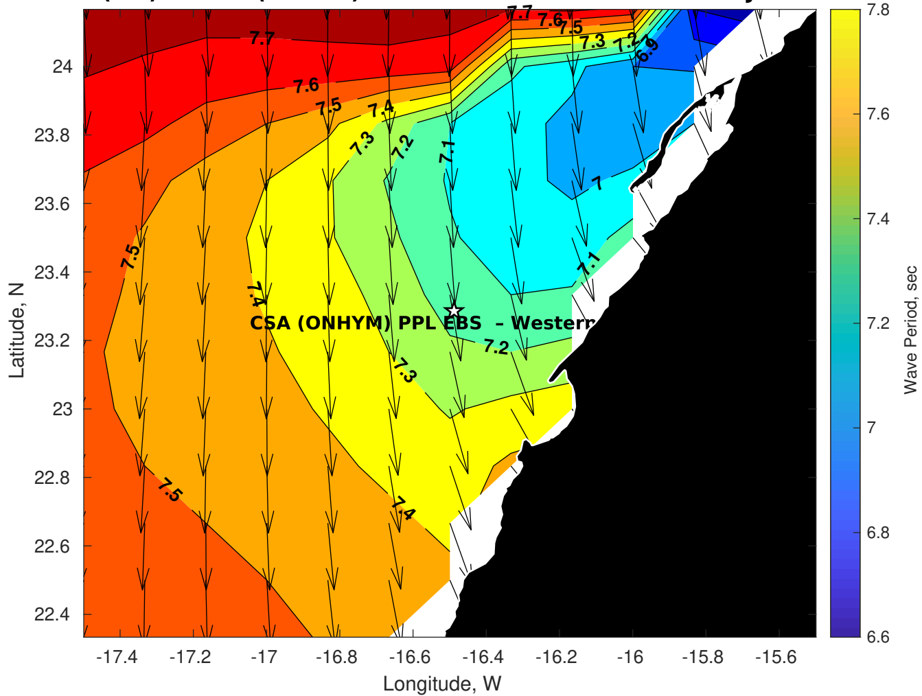
Wave Period (sec) for CSA (ONHYM) PPL EBS - Western Sahara at 25-Jul-2025 21:00:00
