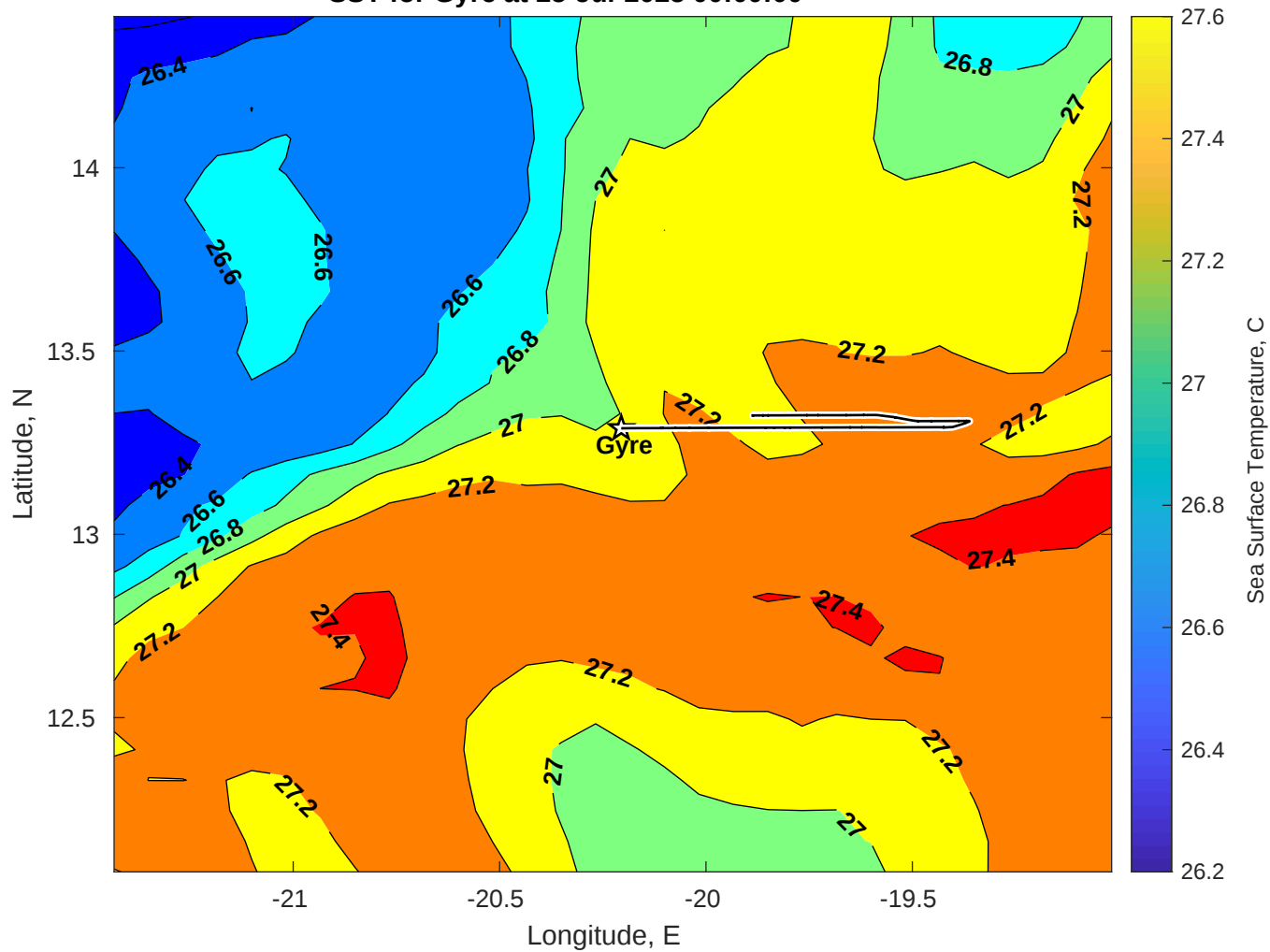
SST for Gyre at 25-Jul-2025 00:00:00
