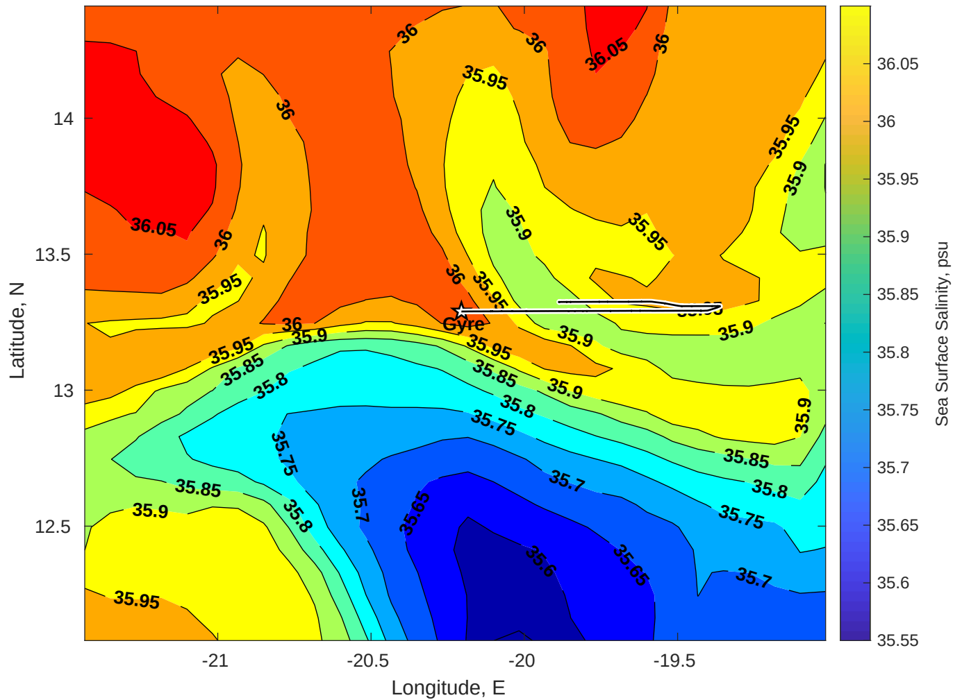
Surface Salinity for Gyre at 25-Jul-2025 00:00:00
