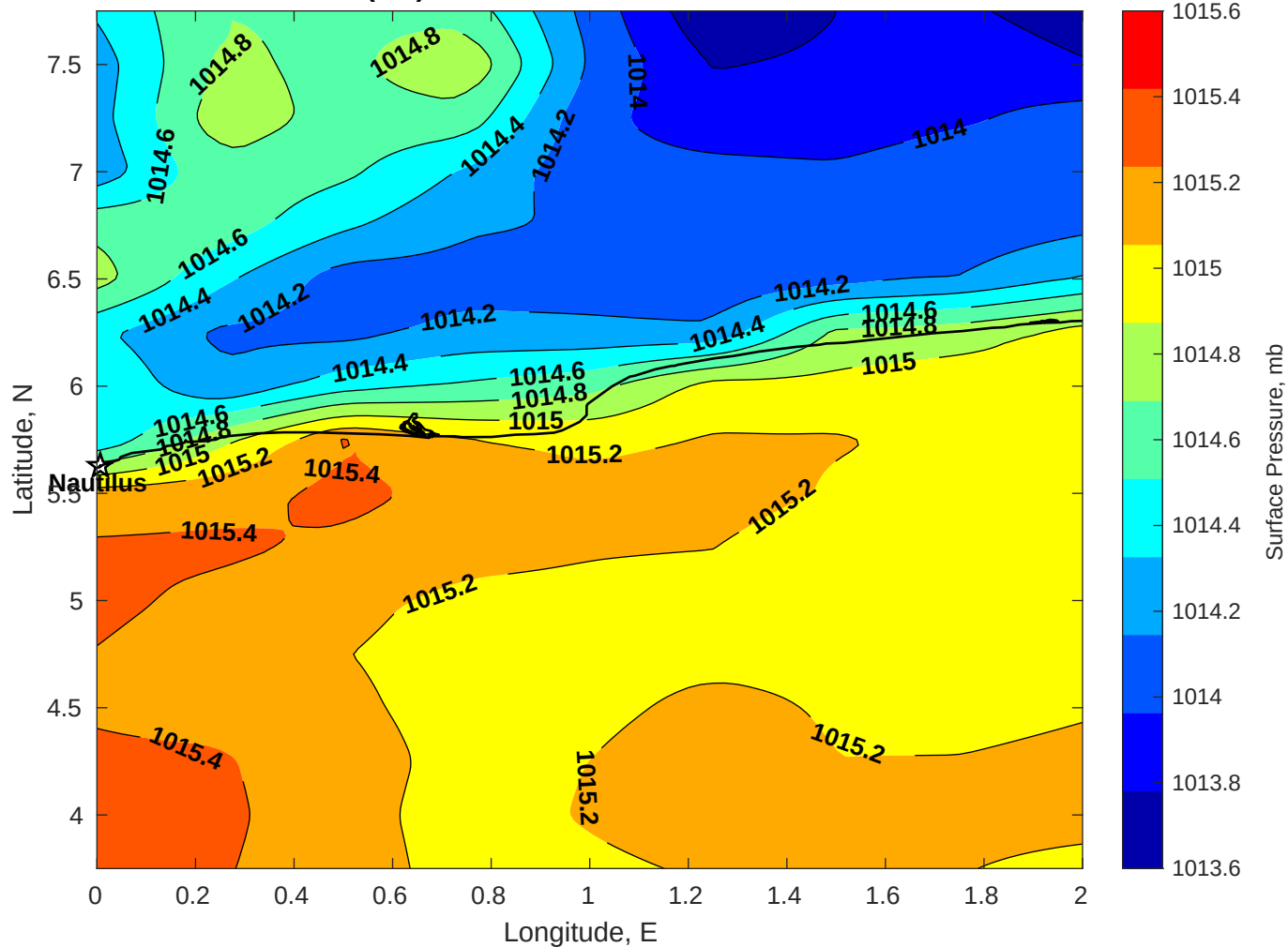
Surface Pressure (mb) for Nautilus at 25-Jul-2025 12:00:00
