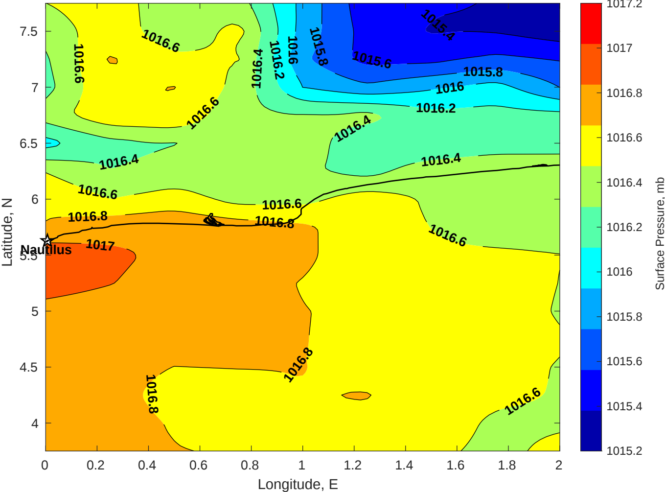
Surface Pressure (mb) for Nautilus at 27-Jul-2025 12:00:00
