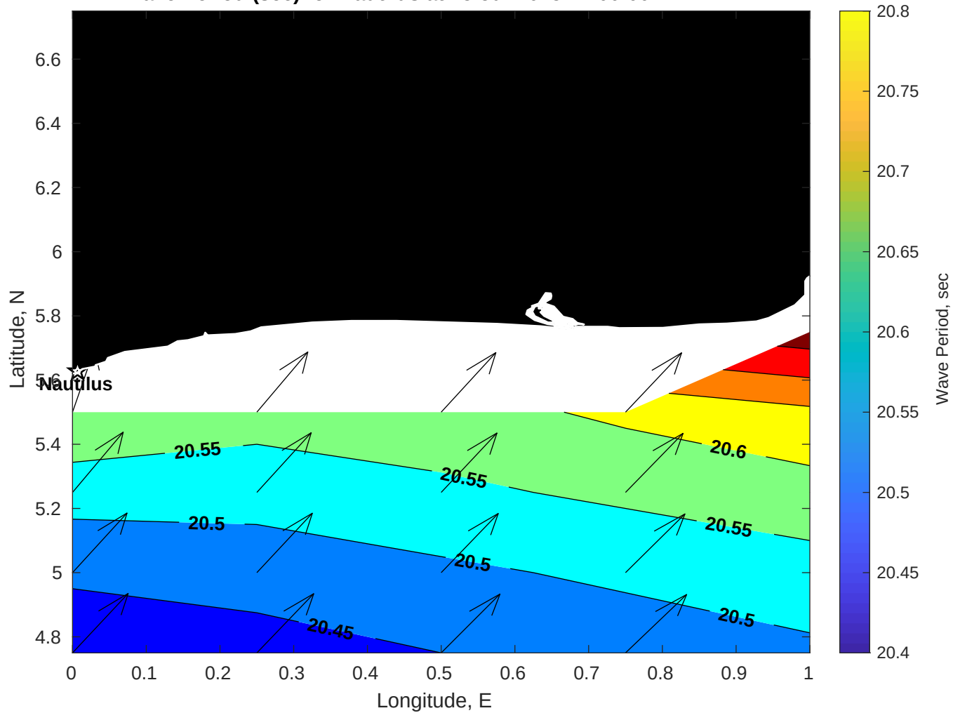
Wave Period (sec) for Nautilus at 25-Jul-2025 21:00:00
