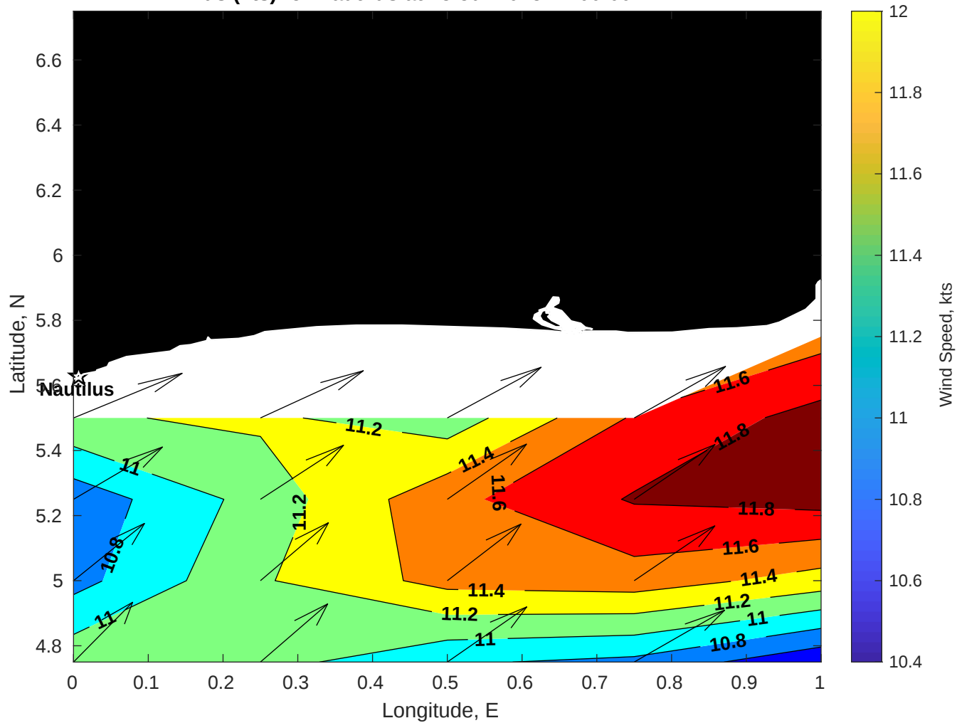
Winds (kts) for Nautilus at 25-Jul-2025 21:00:00
