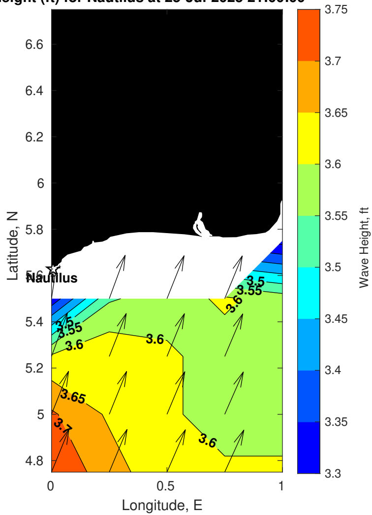
Wave Height (ft) for Nautilus at 25-Jul-2025 21:00:00
