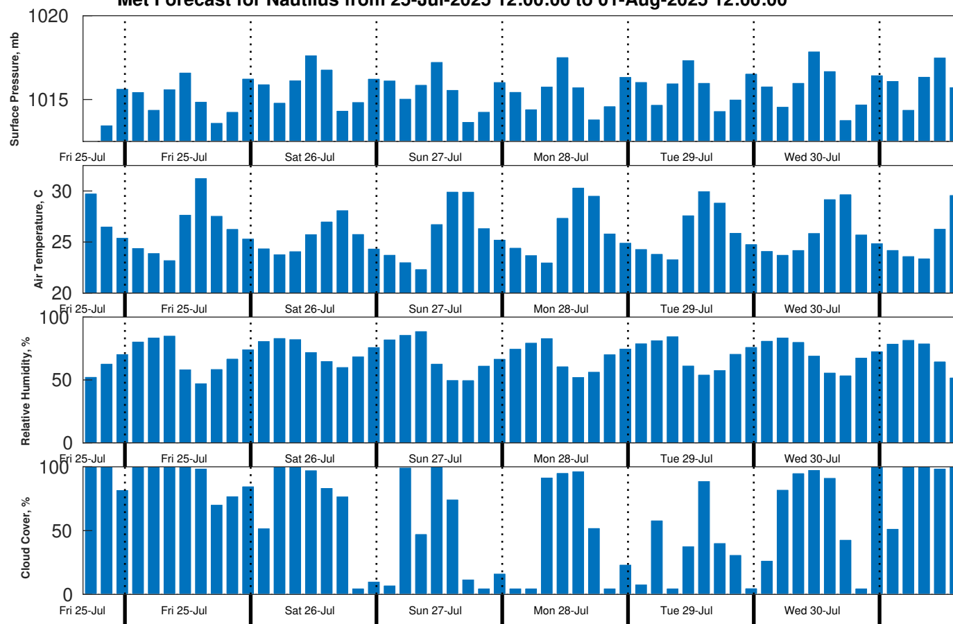
Met Forecast for Nautilus from 25-Jul-2025 12:00:00 to 01-Aug-2025 12:00:00
