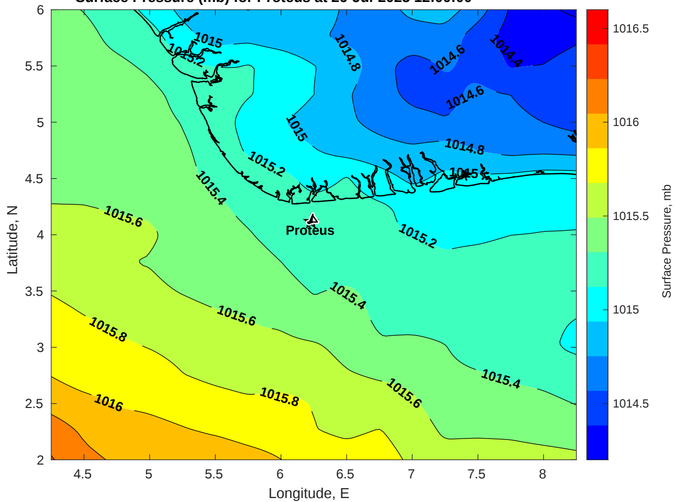
Surface Pressure (mb) for Proteus at 26-Jul-2025 12:00:00
