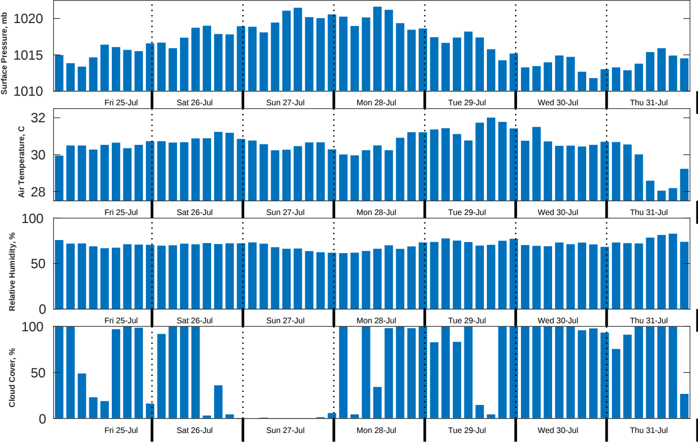
Met Forecast for Shell Noches GC19 PPL Geotechnical from 25-Jul-2025 00:00:00 to 01-Aug-2025 00:00:00
