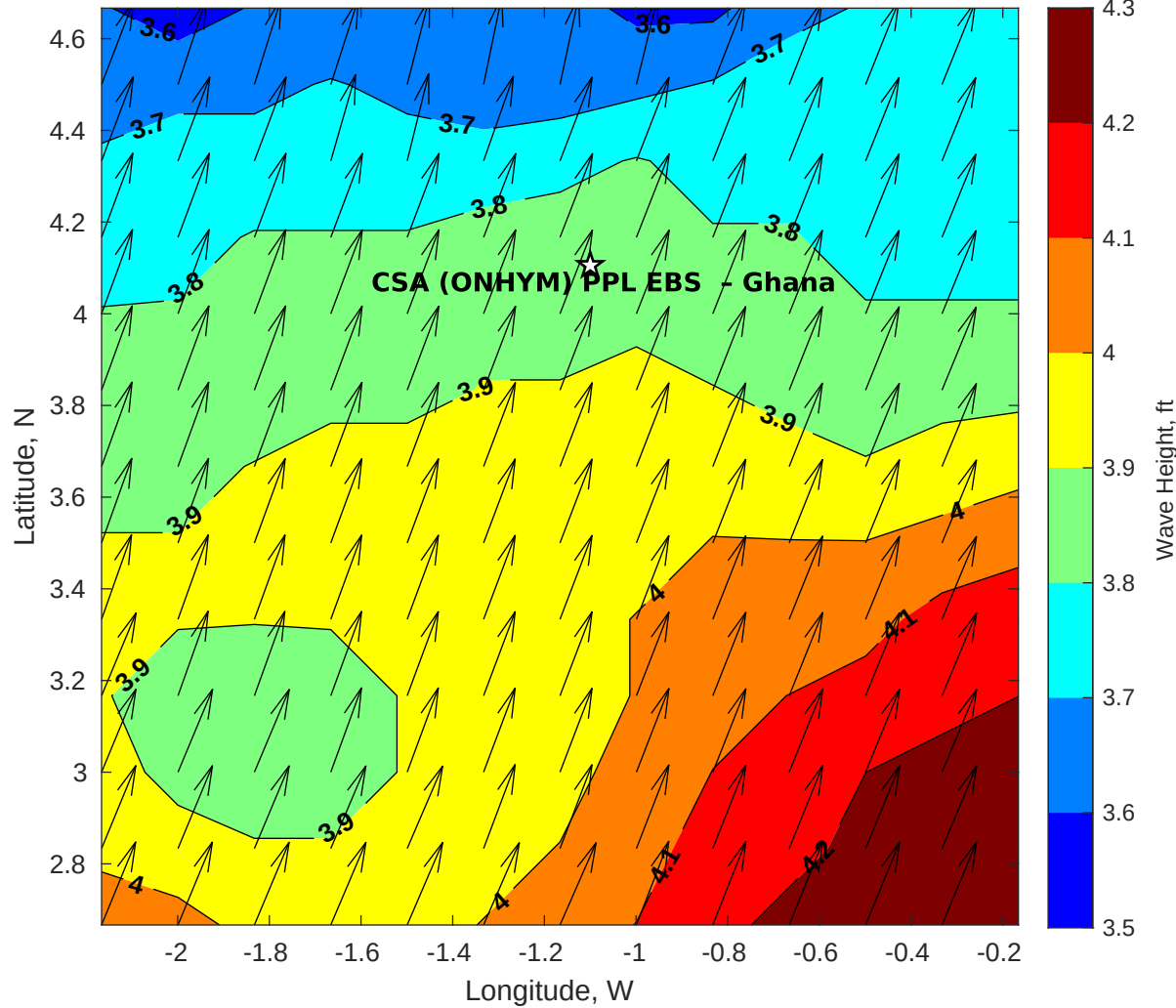
Wave Height (ft) for CSA (ONHYM) PPL EBS - Ghana at 25-Jul-2025 21:00:00
