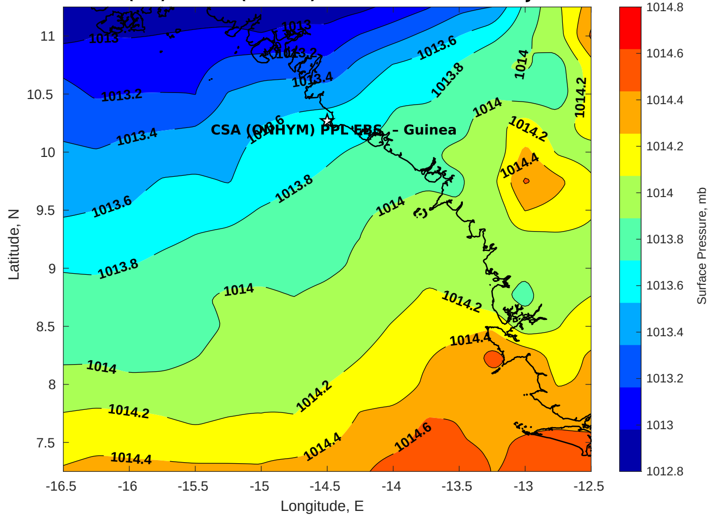
Surface Pressure (mb) for CSA (ONHYM) PPL EBS - Guinea at 25-Jul-2025 12:00:00
